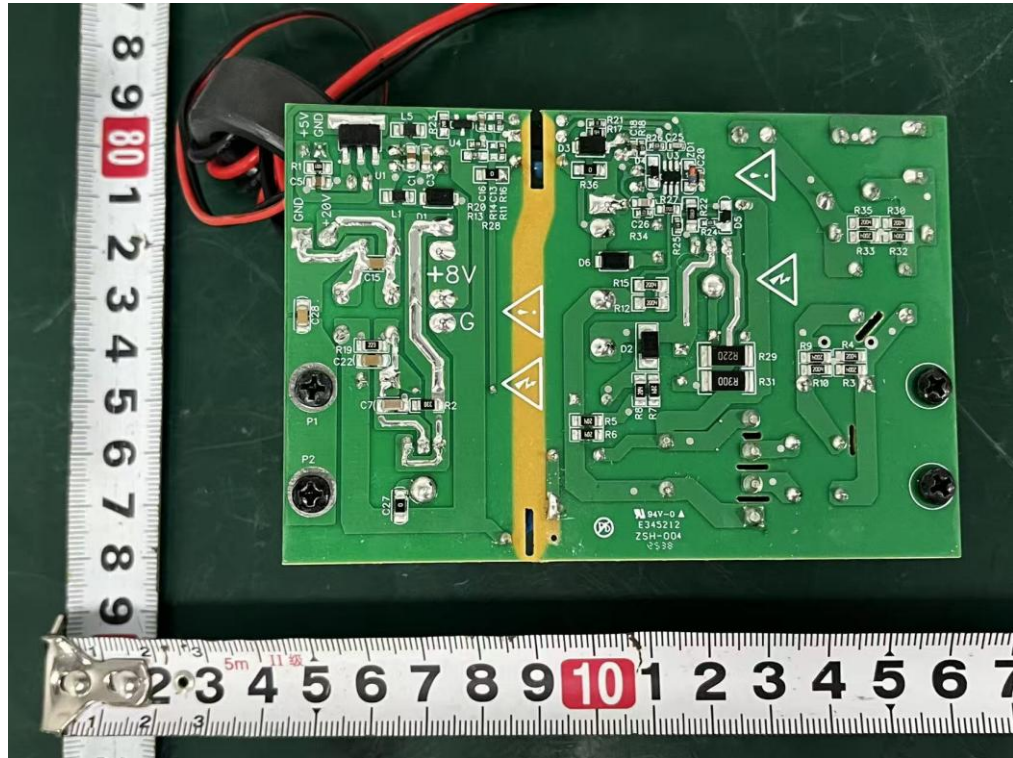
Internal Photos M/N: MediaOne MX5BT
