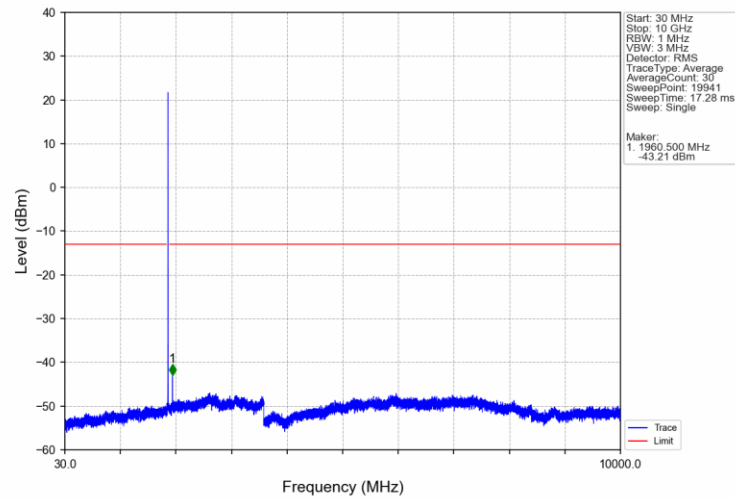
Band2 1.4MHz QPSK MCH 1880MHz RB 1 0 NTN
