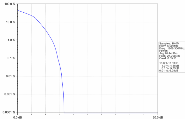
Band2_1.4MHz_16QAM_HCH_1909.3MHz_RB_6_0_NTNV
