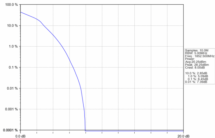
Band2_5MHz_16QAM_LCH_1852.5MHz_RB_25_0_NTNV
