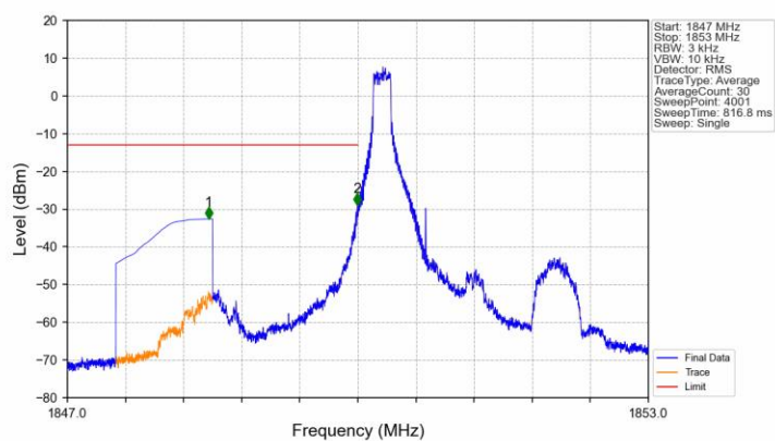
Band2_1.4MHz_QPSK_LCH_1850.7MHz_RB_1_0_NTNV
