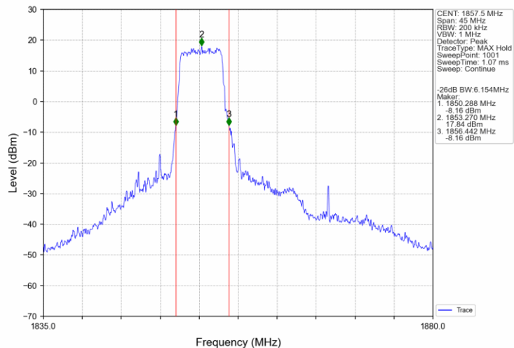
Band2_15MHz_16QAM_LCH_1857.5MHz_RB_27_0_NTNV
