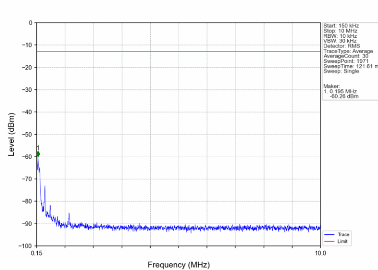
Band2_1.4MHz_16QAM_LCH_1850.7MHz_RB_1_0_NTNV
