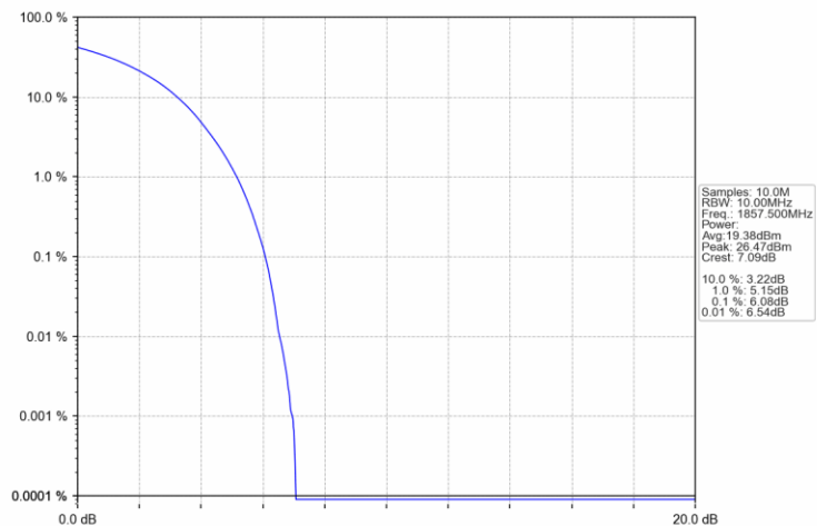
Band2_15MHz_16QAM_LCH_1857.5MHz_RB_27_0_NTNV
