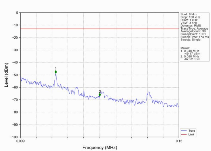
Band2_1.4MHz_16QAM_LCH_1850.7MHz_RB_1_0_NTNV
