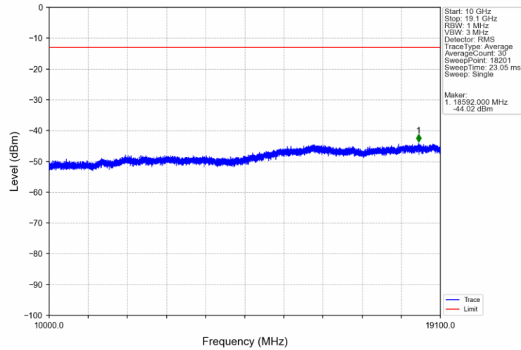
Band2_5MHz_16QAM_LCH_1852.5MHz_RB_25_0_NTNV
