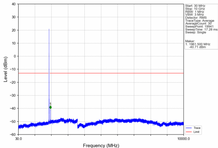
Band2_5MHz_16QAM_MCH_1880MHz_RB_1_0_NTNV
