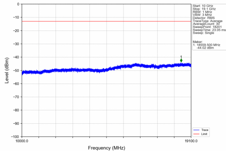
Band2_5MHz_QPSK_LCH_1852.5MHz_RB_1_0_NTNV
