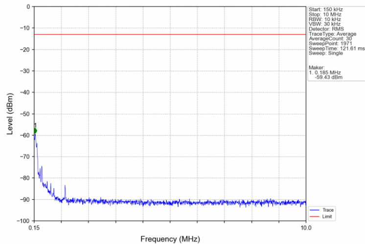
Band2_5MHz_QPSK_HCH_1907.5MHz_RB_1_0_NTNV
