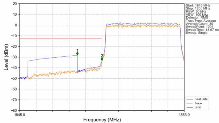
Band2_5MHz_16QAM_LCH_1852.5MHz_RB_25_0_NTNV
