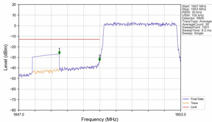
Band2_3MHz_16QAM_LCH_1851.5MHz_RB_15_0_NTNV
