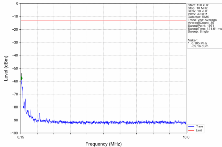
Band2_5MHz_16QAM_MCH_1880MHz_RB_1_0_NTNV
