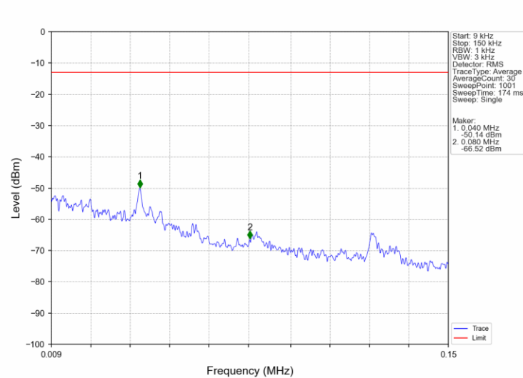
Band2_1.4MHz_16QAM_HCH_1909.3MHz_RB_1_0_NTNV
