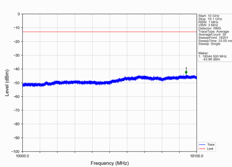
Band2_1.4MHz_16QAM_MCH_1880MHz_RB_1_0_NTNV
