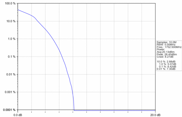
Band4_5MHz_16QAM_HCH_1752.5MHz_RB_25_0_NTNV
