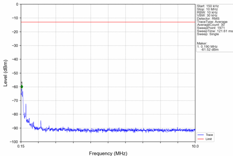
Band4_1.4MHz_QPSK_HCH_1754.3MHz_RB_1_0_NTNV
