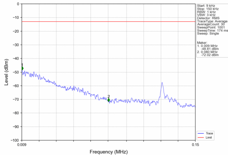
Band4_3MHz_QPSK_LCH_1711.5MHz_RB_1_0_NTNV
