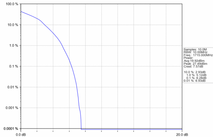
Band4_10MHz_16QAM_LCH_1715MHz_RB_27_0_NTNV
