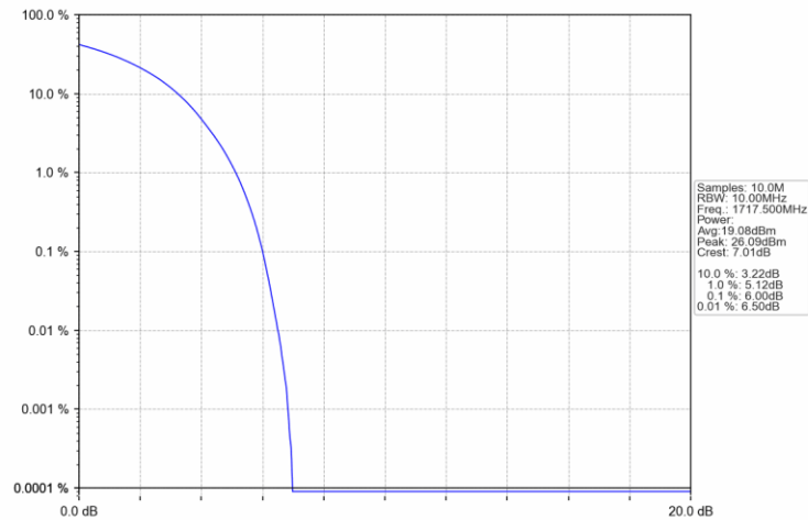
Band4_15MHz_16QAM_LCH_1717.5MHz_RB_27_0_NTNV
