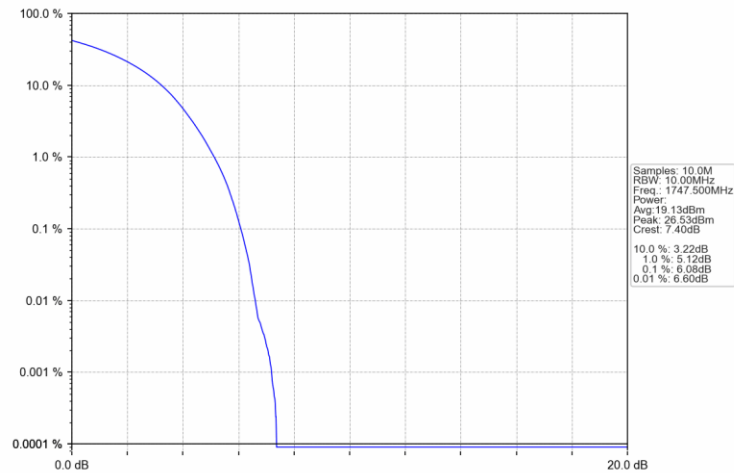
Band4_15MHz_16QAM_HCH_1747.5MHz_RB_27_48_NTNV
