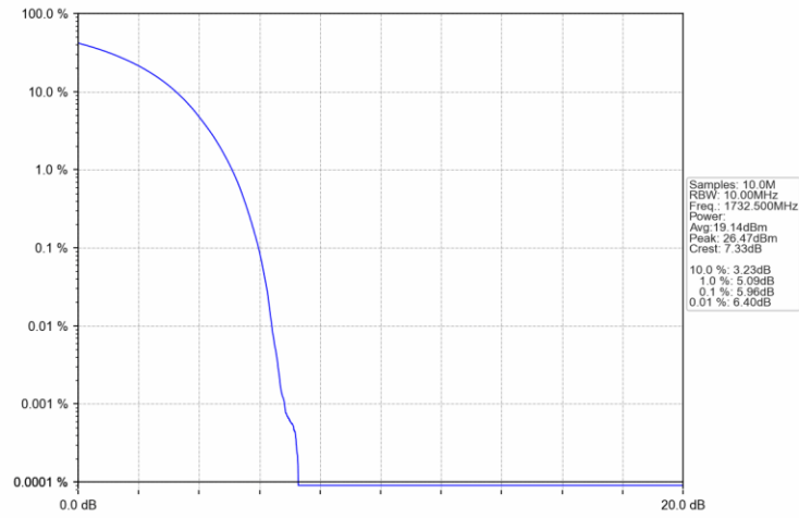
Band4_15MHz_16QAM_MCH_1732.5MHz_RB_27_0_NTNV
