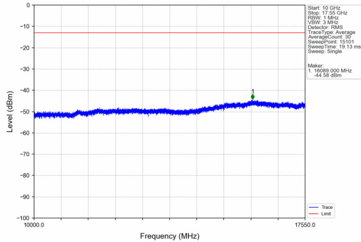
Band4_1.4MHz_QPSK_HCH_1754.3MHz_RB_1_5_NTNV
