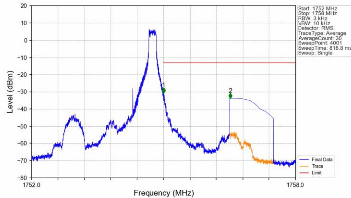
Band4_1.4MHz_QPSK_HCH_1754.3MHz_RB_1_5_NTNV
