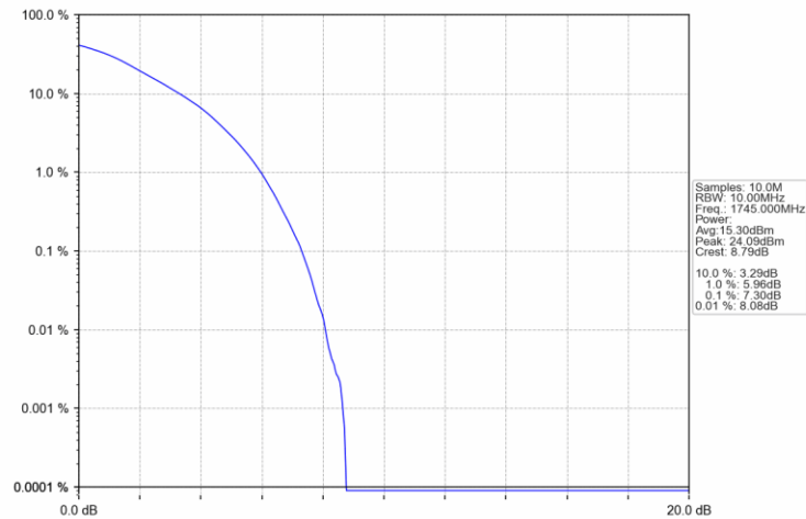
Band4_20MHz_16QAM_HCH_1745MHz_RB_27_73_NTNV
