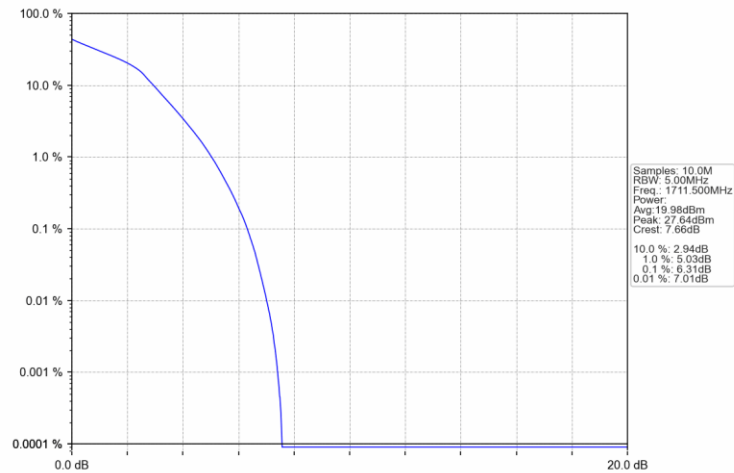
Band4_3MHz_16QAM_LCH_1711.5MHz_RB_15_0_NTNV
