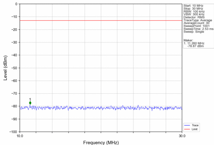
Band4_1.4MHz_QPSK_LCH_1710.7MHz_RB_1_0_NTNV
