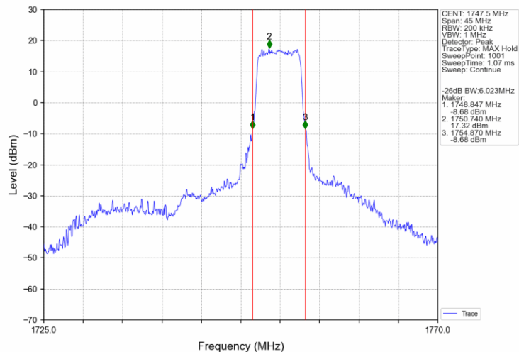
Band4_15MHz_16QAM_HCH_1747.5MHz_RB_27_48_NTNV
