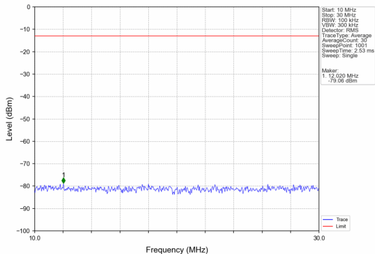
Band4_10MHz_QPSK_MCH_1732.5MHz_RB_1_0_NTNV
