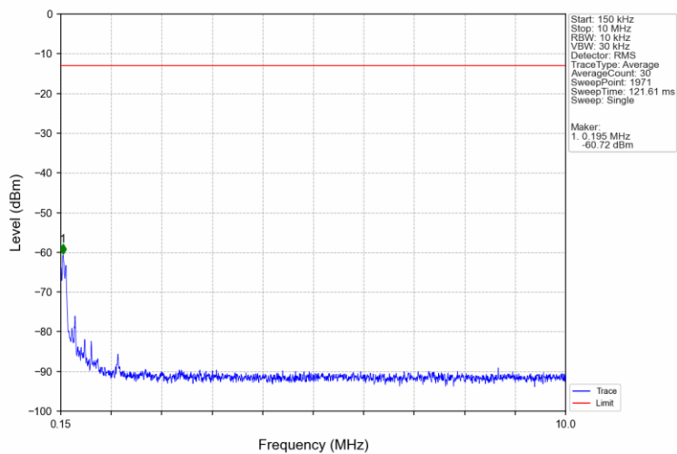
Band4_3MHz_QPSK_MCH_1732.5MHz_RB_1_0_NTNV
