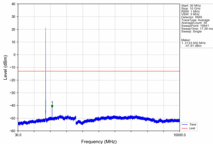
Band4_5MHz_16QAM_MCH_1732.5MHz_RB_1_0_NTNV
