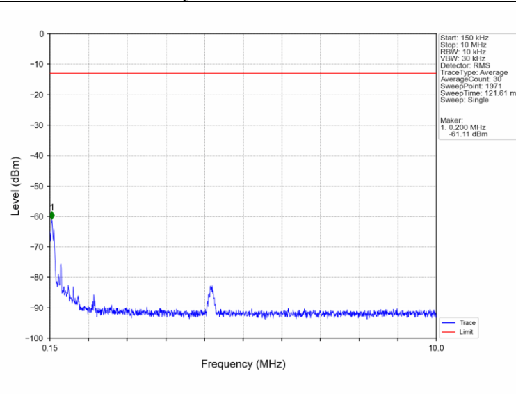
Band4_5MHz_16QAM_LCH_1712.5MHz_RB_1_0_NTNV
