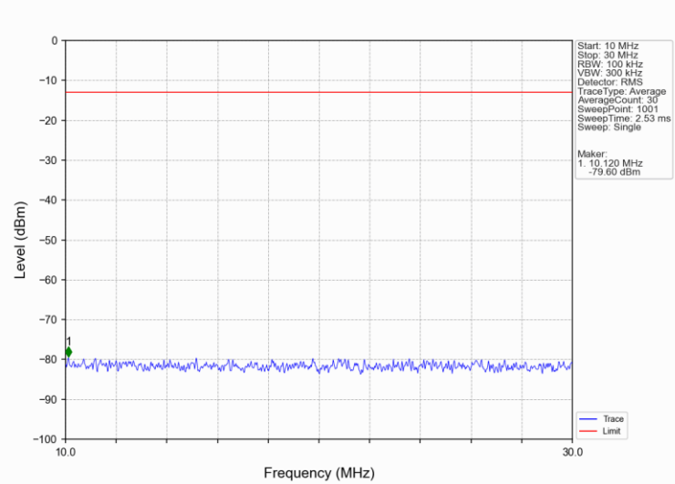
Band4_3MHz_16QAM_MCH_1732.5MHz_RB_1_0_NTNV
