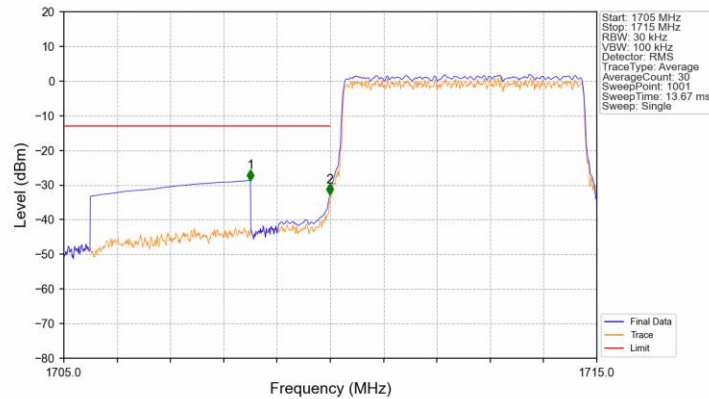
Band4_5MHz_16QAM_LCH_1712.5MHz_RB_25_0_NTNV
