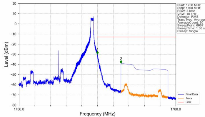
Band4_5MHz_QPSK_HCH_1752.5MHz_RB_1_24_NTNV
