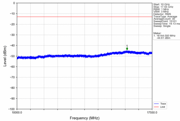
Band4_5MHz_QPSK_HCH_1752.5MHz_RB_1_24_NTNV
