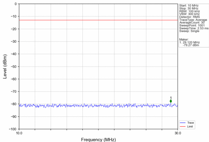
Band4_5MHz_QPSK_MCH_1732.5MHz_RB_1_0_NTNV
