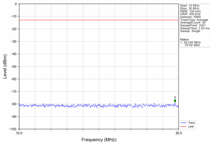
Band4_3MHz_QPSK_MCH_1732.5MHz_RB_1_0_NTNV
