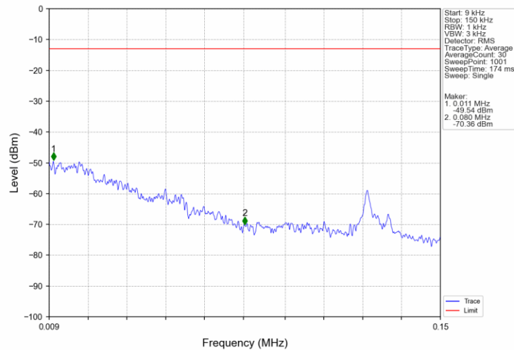
Band4_5MHz_QPSK_LCH_1712.5MHz_RB_1_0_NTNV
