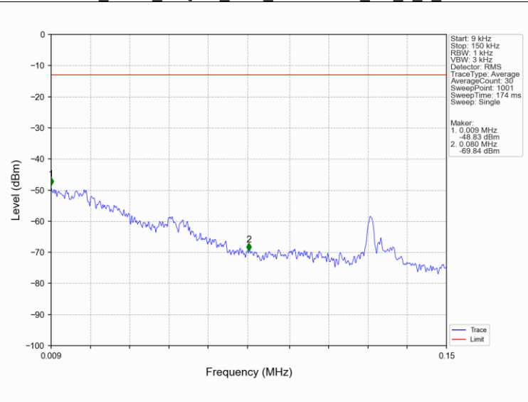
Band4_5MHz_16QAM_LCH_1712.5MHz_RB_1_0_NTNV
