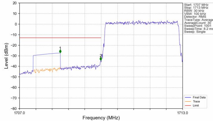
Band4_3MHz_16QAM_LCH_1711.5MHz_RB_15_0_NTNV
