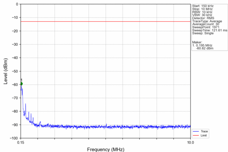
Band4_3MHz_QPSK_HCH_1753.5MHz_RB_1_0_NTNV
