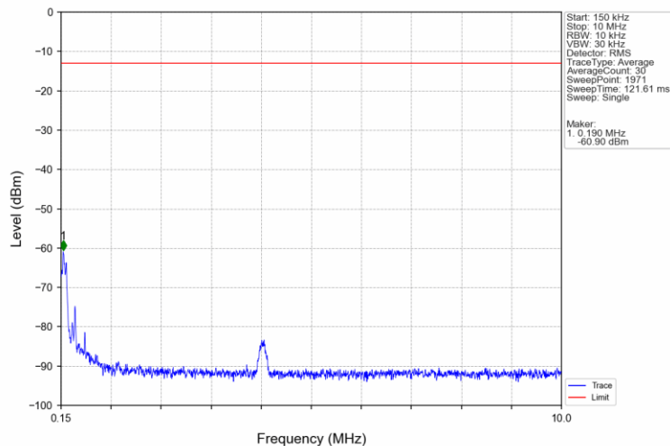
Band4_3MHz_16QAM_LCH_1711.5MHz_RB_1_0_NTNV
