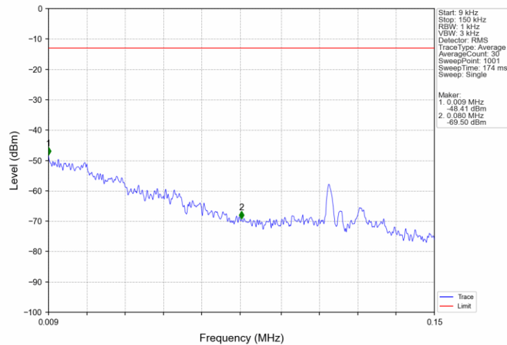
Band4_10MHz_QPSK_LCH_1715MHz_RB_1_0_NTNV
