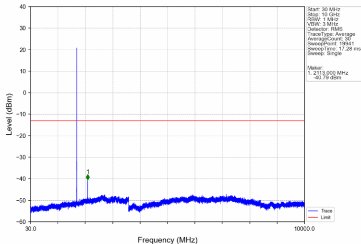
Band4_3MHz_16QAM_LCH_1711.5MHz_RB_1_0_NTNV
