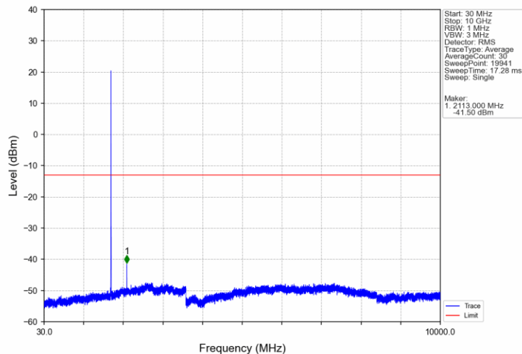
Band4_5MHz_16QAM_LCH_1712.5MHz_RB_1_0_NTNV
