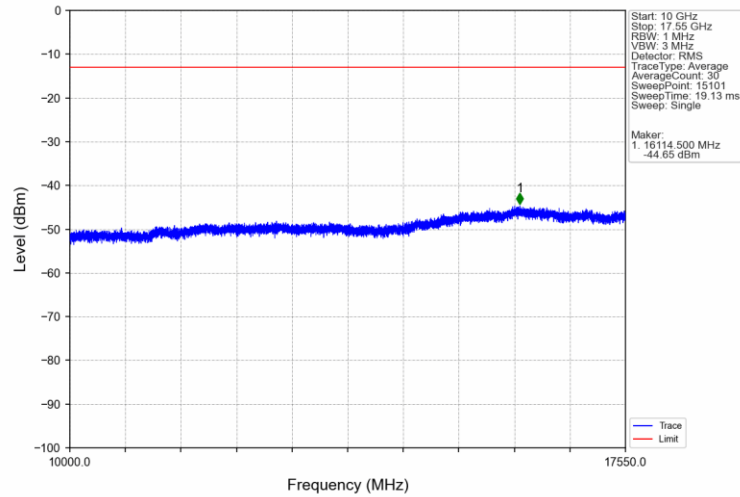
Band4_5MHz_16QAM_LCH_1712.5MHz_RB_25_0_NTNV
