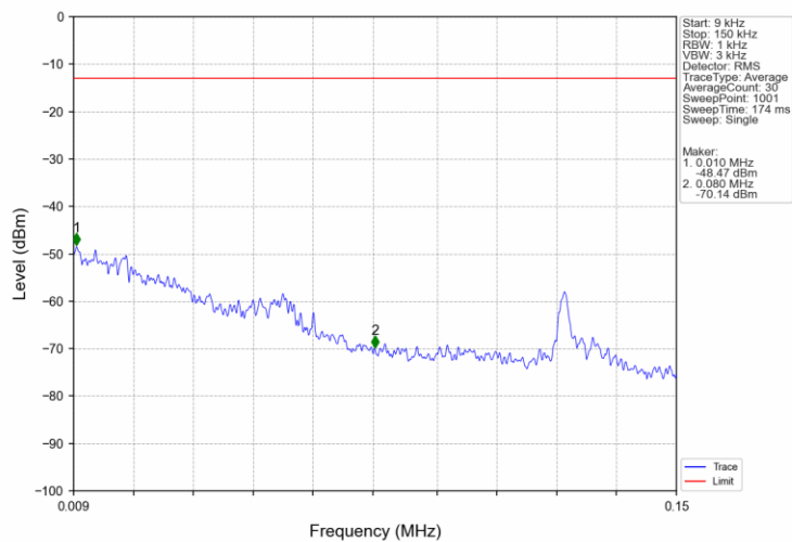
Band4_3MHz_QPSK_HCH_1753.5MHz_RB_1_0_NTNV
