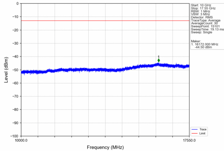
Band4_5MHz_QPSK_MCH_1732.5MHz_RB_1_0_NTNV
