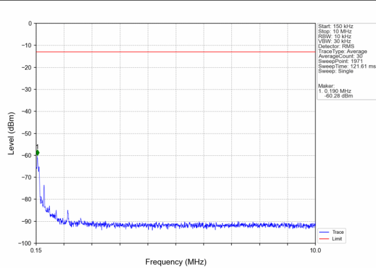
Band4_20MHz_16QAM_HCH_1745MHz_RB_1_0_NTNV
