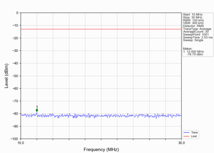
Band4_20MHz_16QAM_HCH_1745MHz_RB_1_0_NTNV
