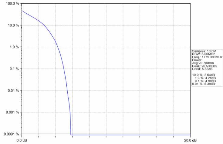
Band66_1.4MHz_QPSK_HCH_1779.3MHz_RB_6_0_NTNV
