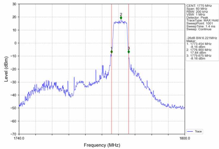
Band66_20MHz_16QAM_HCH_1770MHz_RB_27_73 NTN
