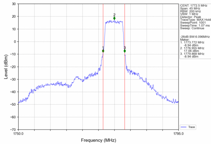
Band66_15MHz_16QAM_HCH_1772.5MHz_RB_27_48_NTNV
