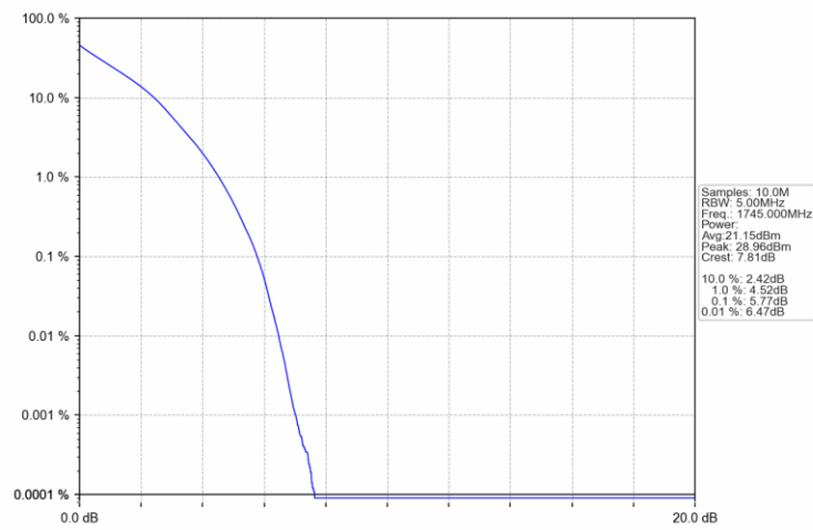
Band66_5MHz_QPSK_MCH_1745MHz_RB_25_0_NTNV
