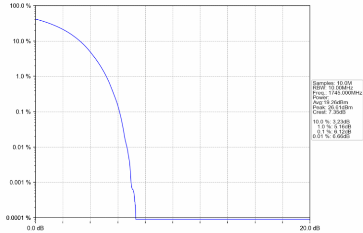
Band66_15MHz_16QAM_MCH_1745MHz_RB_27_0_NTNV
