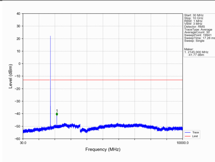
Band66_5MHz_QPSK_MCH_1745MHz_RB_1_0_NTNV
