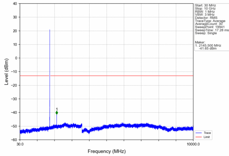
Band66_3MHz_QPSK_MCH_1745MHz_RB_1_0_NTNV
