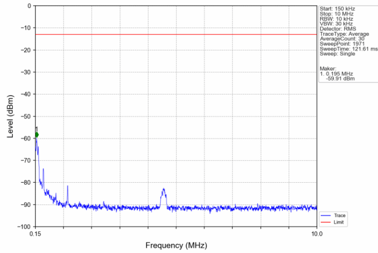
Band66_10MHz_QPSK_LCH_1715MHz_RB_1_0_NTNV
