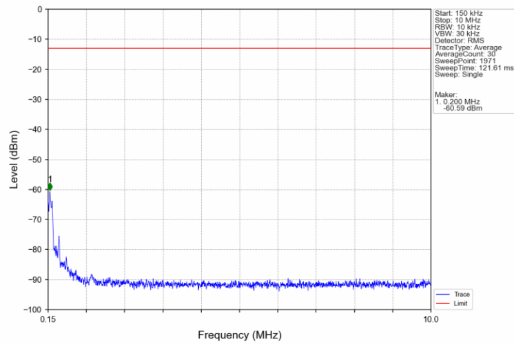
Band66_5MHz_QPSK_HCH_1777.5MHz_RB_1_0_NTNV
