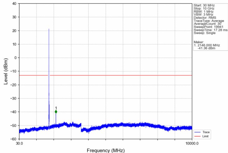
Band66_10MHz_QPSK_MCH_1745MHz_RB_1_0_NTNV
