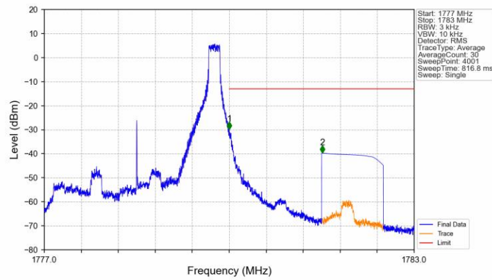
Band66_3MHz_QPSK_HCH_1778.5MHz_RB_1_14_NTNV
