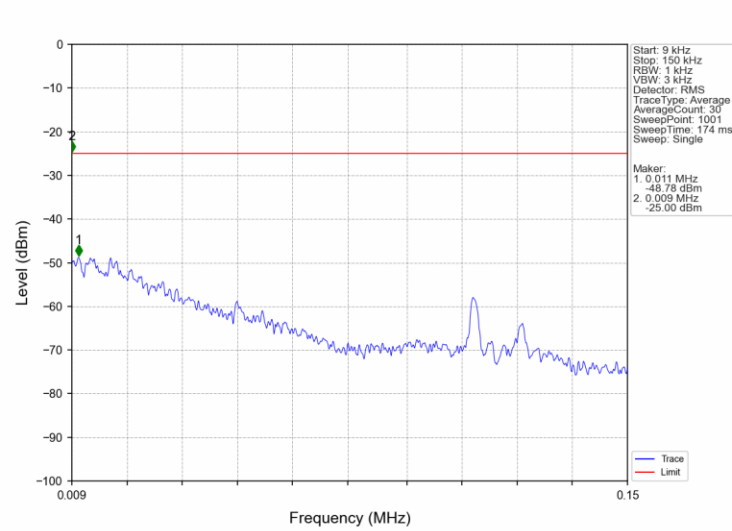
Band7_15MHz_16QAM_MCH_2535MHz_RB_1_0_NTNV
