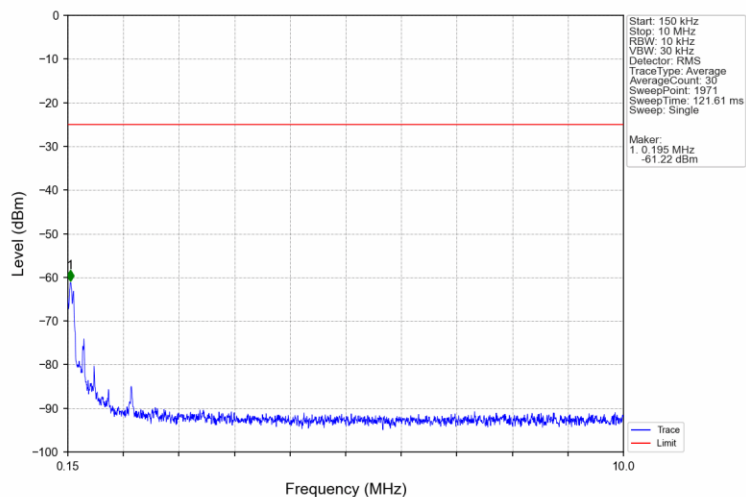
Band7_10MHz_16QAM_MCH_2535MHz_RB_1_0_NTNV
