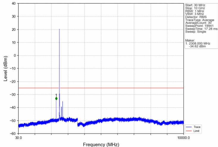
Band7_15MHz_QPSK_LCH_2507.5MHz_RB_1_0_NTNV
