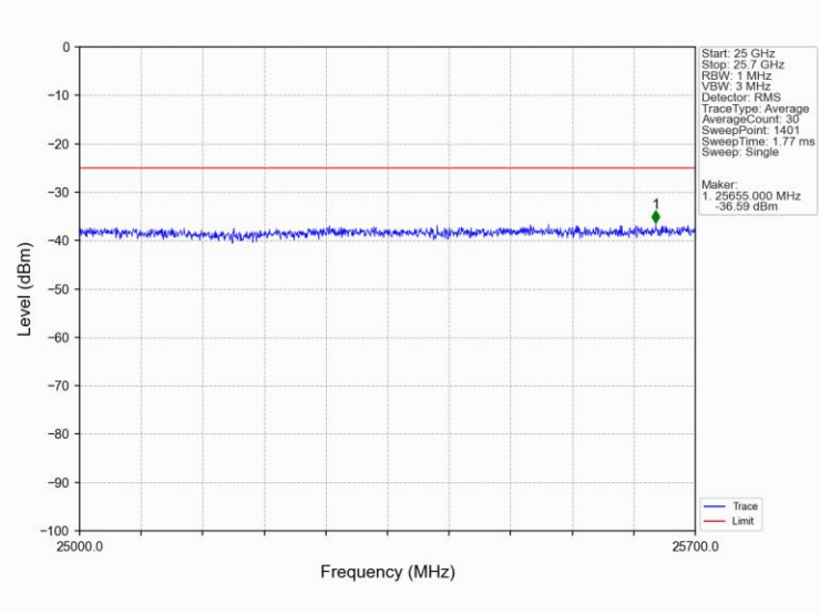
Band7_15MHz_16QAM_MCH_2535MHz_RB_1_0_NTNV
