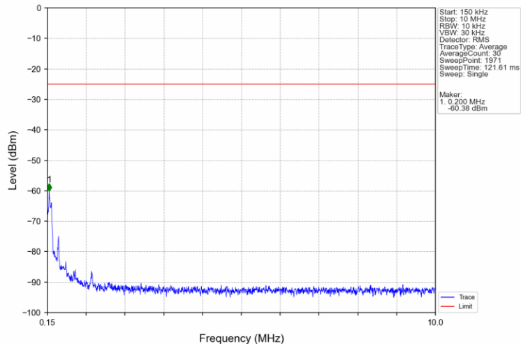
Band7_15MHz_16QAM_MCH_2535MHz_RB_1_0_NTNV
