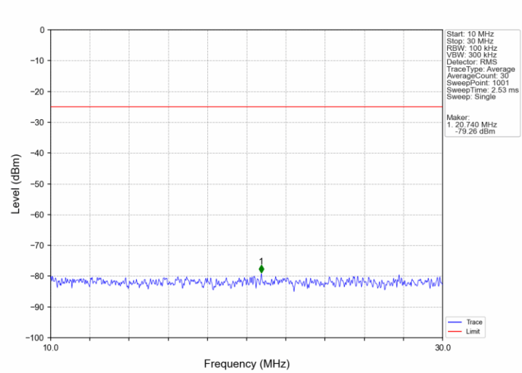
Band7_10MHz_16QAM_HCH_2565MHz_RB_1_0_NTNV
