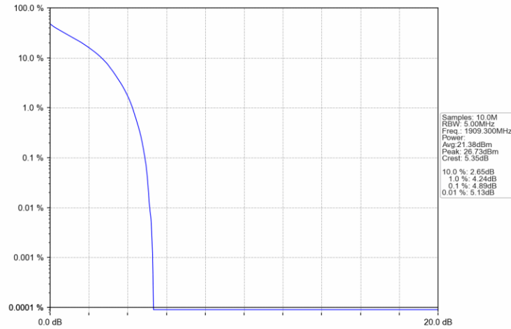
Band2_1.4MHz_QPSK_HCH_1909.3MHz_RB_6_0_NTNV
