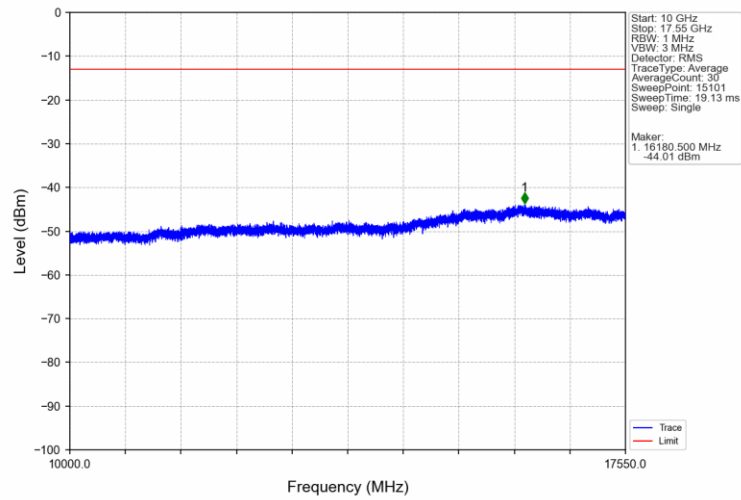
Band4_1.4MHz_QPSK_HCH_1754.3MHz_RB_1_5_NTNV
