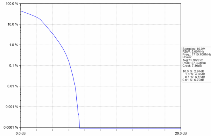
Band4_1.4MHz_16QAM_LCH_1710.7MHz_RB_6_0_NTNV
