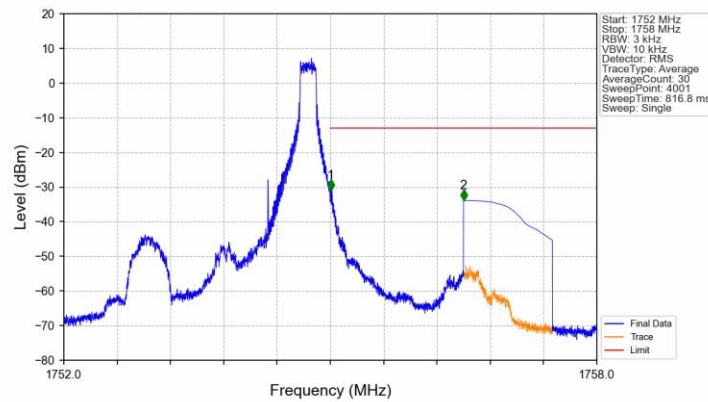
Band4_1.4MHz_QPSK_HCH_1754.3MHz_RB_1_5_NTNV
