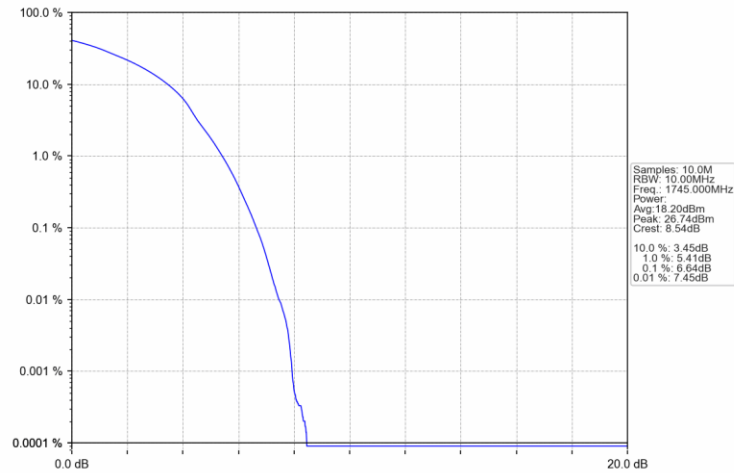
Band4_20MHz_16QAM_HCH_1745MHz_RB_100_0_NTNV
