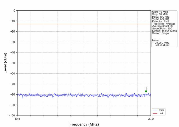
Band5_1.4MHz_16QAM_LCH_824.7MHz_RB_1_0_NTNV
