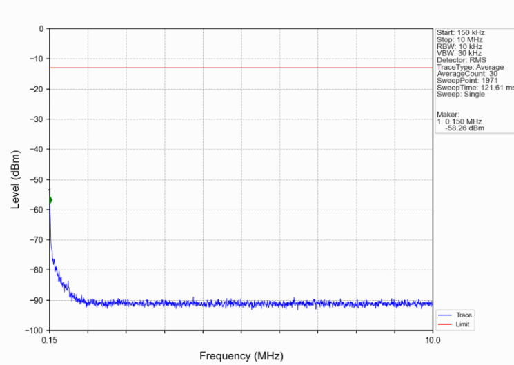
Band5_5MHz_16QAM_LCH_826.5MHz_RB_1_0_NTNV
