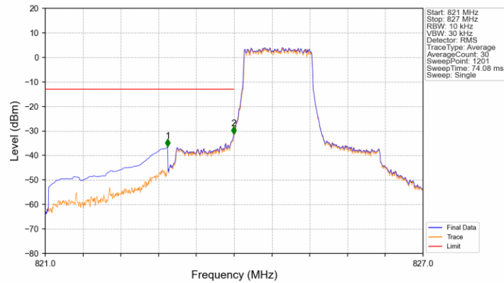
Band5_1.4MHz_QPSK_LCH_824.7MHz_RB_6_0_NTNV
