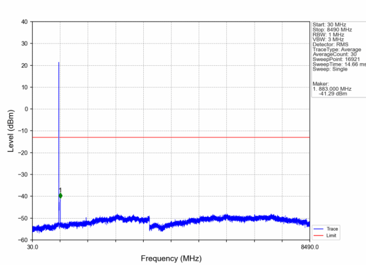
Band5_5MHz_16QAM_MCH_836.5MHz_RB_1_0_NTNV
