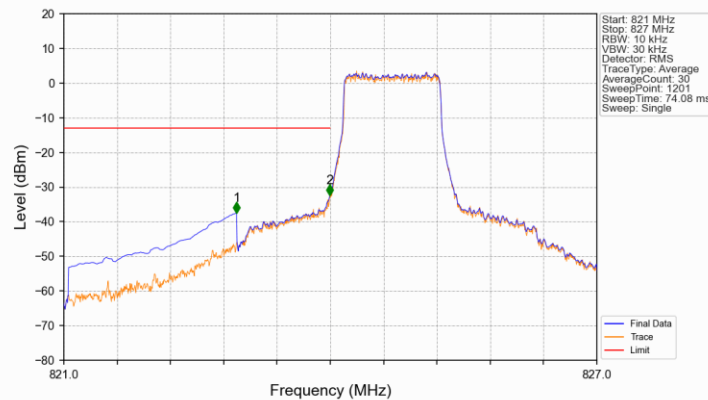
Band5_1.4MHz_16QAM_LCH_824.7MHz_RB_6_0_NTNV
