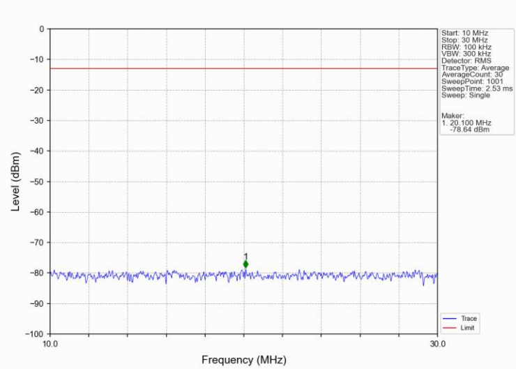
Band5_5MHz_16QAM_MCH_836.5MHz_RB_1_0_NTNV
