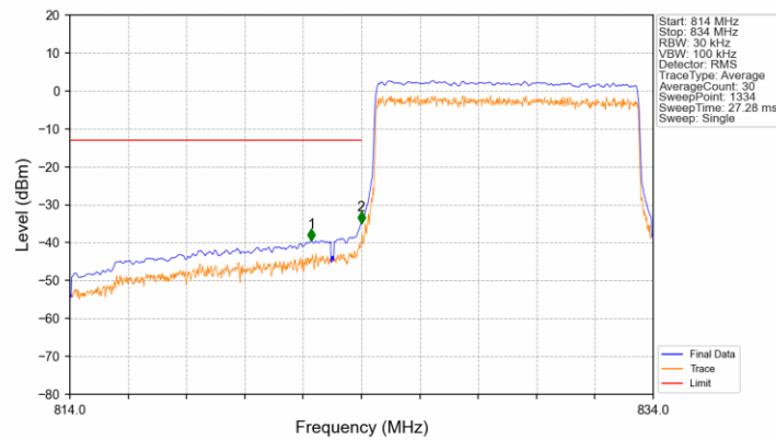
Band5_10MHz_16QAM_LCH_829MHz_RB_50_0_NTNV
