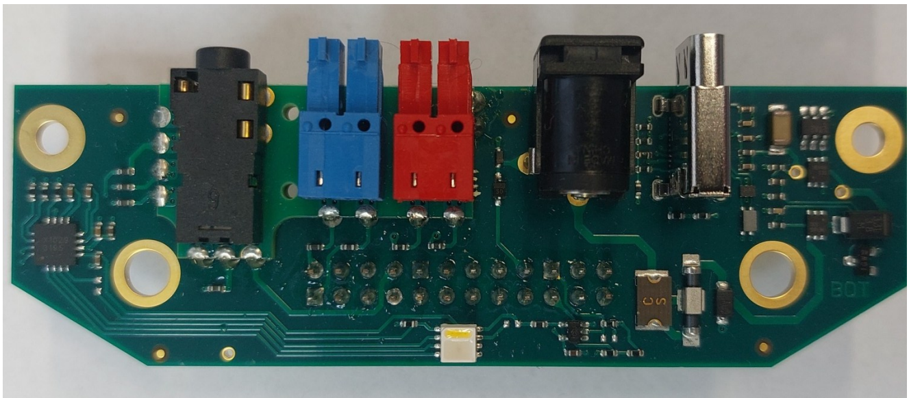
Figure 8 Connector PCBA - Bottom View
