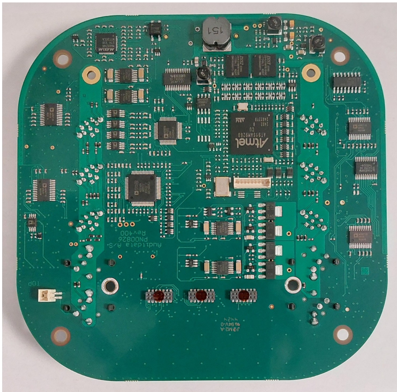
Figure 3 Main PCBA - Top View
