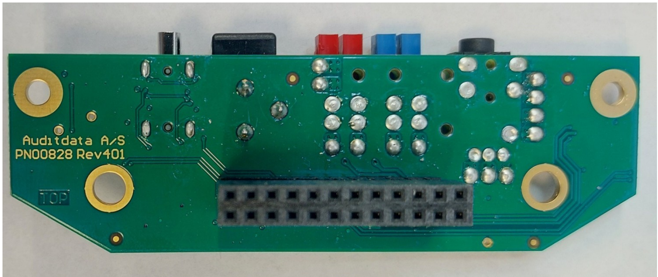
Figure 7 Connector PCBA - Top View
