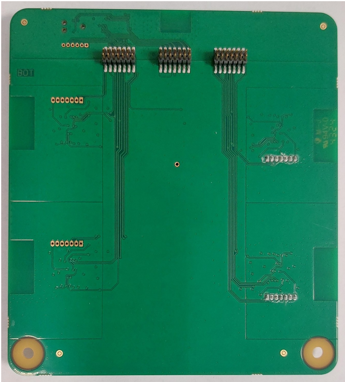
Figure 6 Wireless PCBA - Bottom View
