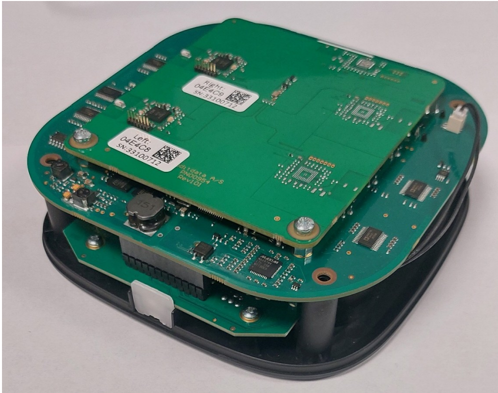
Figure 1 PN00887 Internal Assembly
