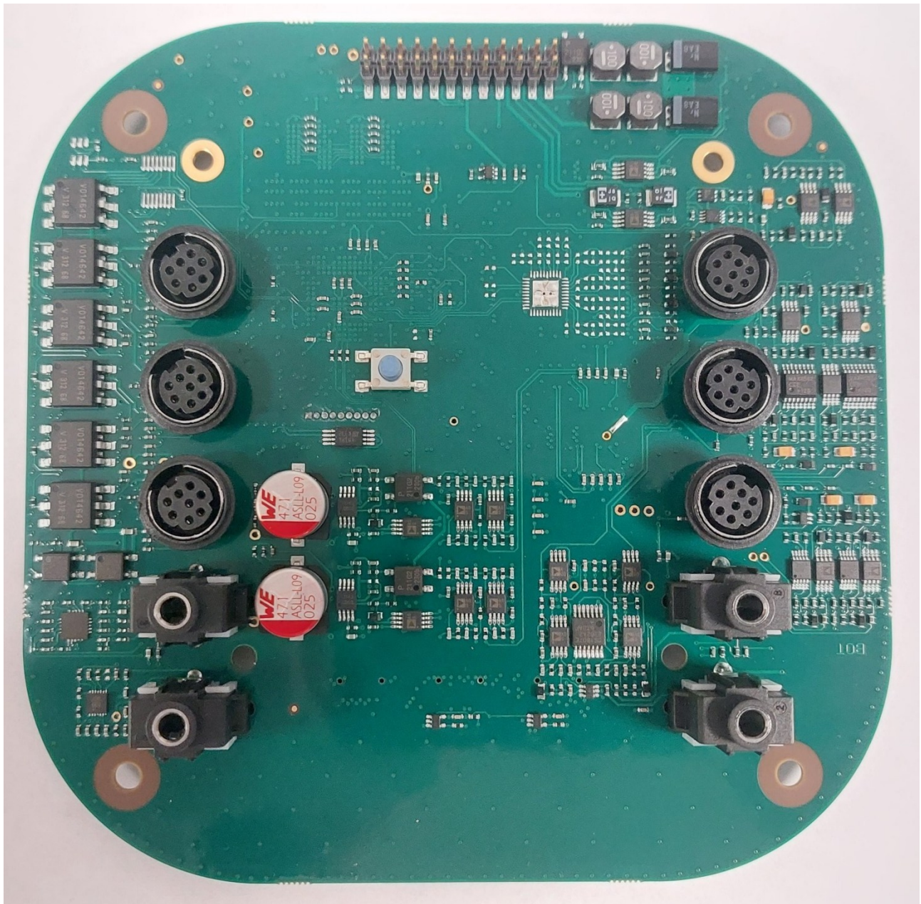
Figure 4 Main PCBA - Bottom View
