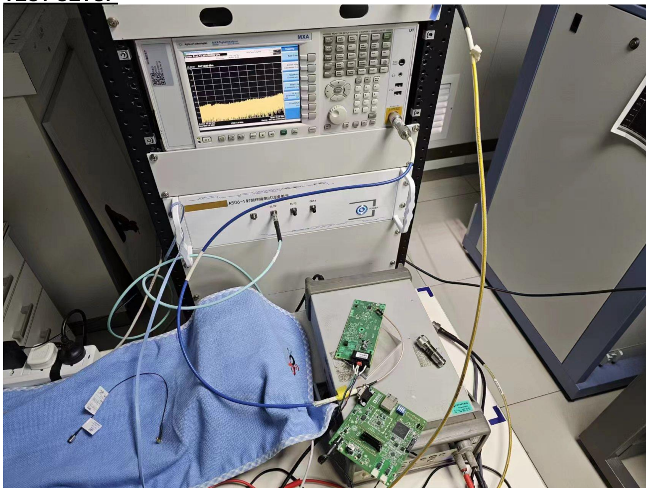
RF Conducted Test setup (2.4G)
