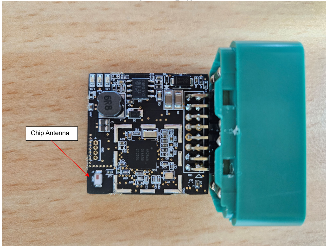
[Main board_Top]
