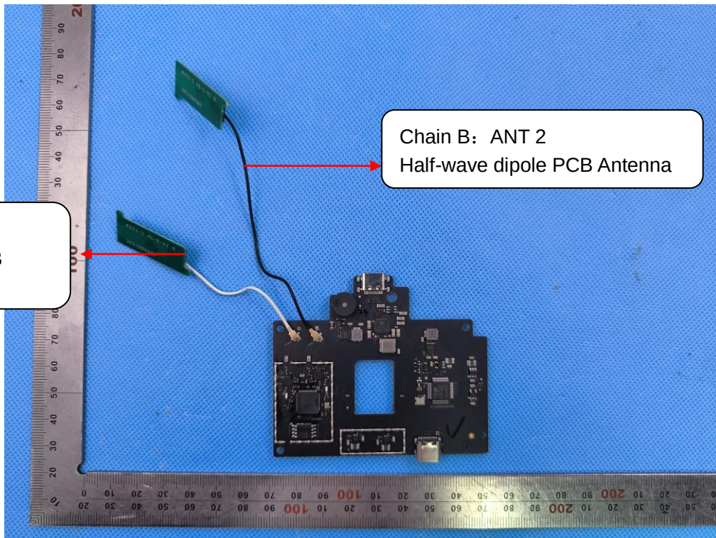
INTERNAL VIEW OF EUT-1 (FIGURE 1)
