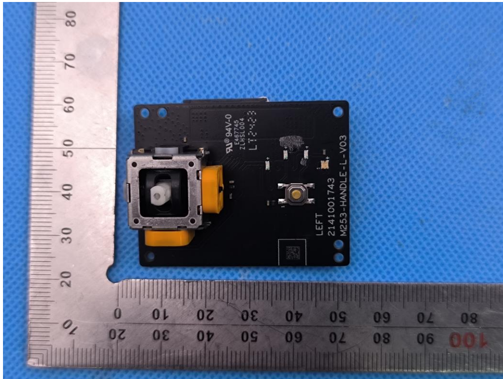
INTERNAL VIEW OF EUT-1 (FIGURE 13)
