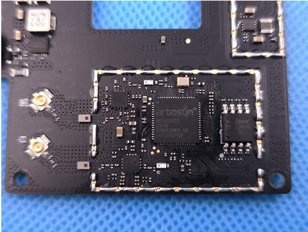
INTERNAL VIEW OF EUT-1 (FIGURE 5)
