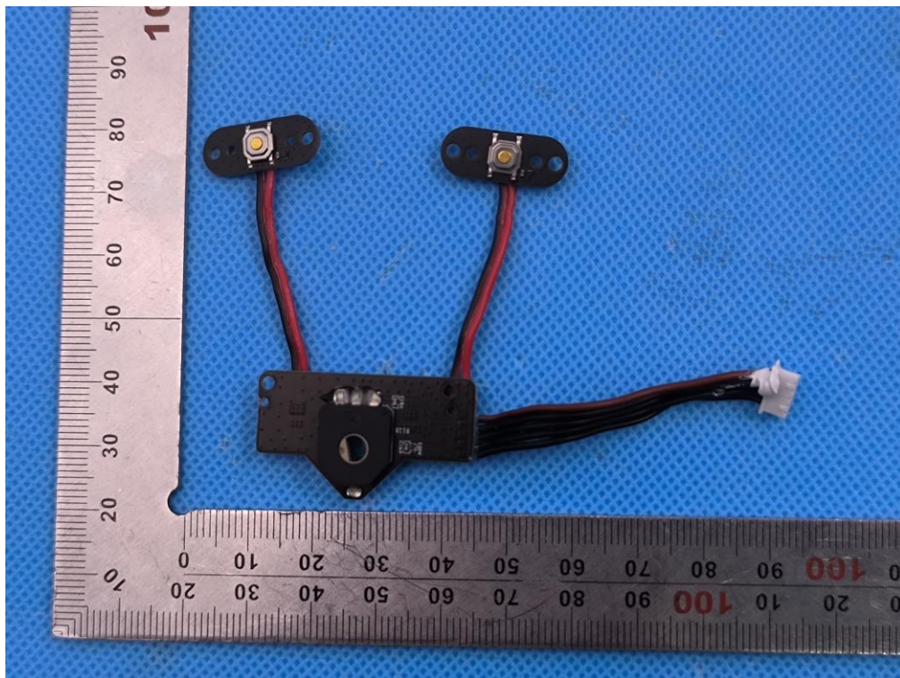
INTERNAL VIEW OF EUT-1 (FIGURE 15)
