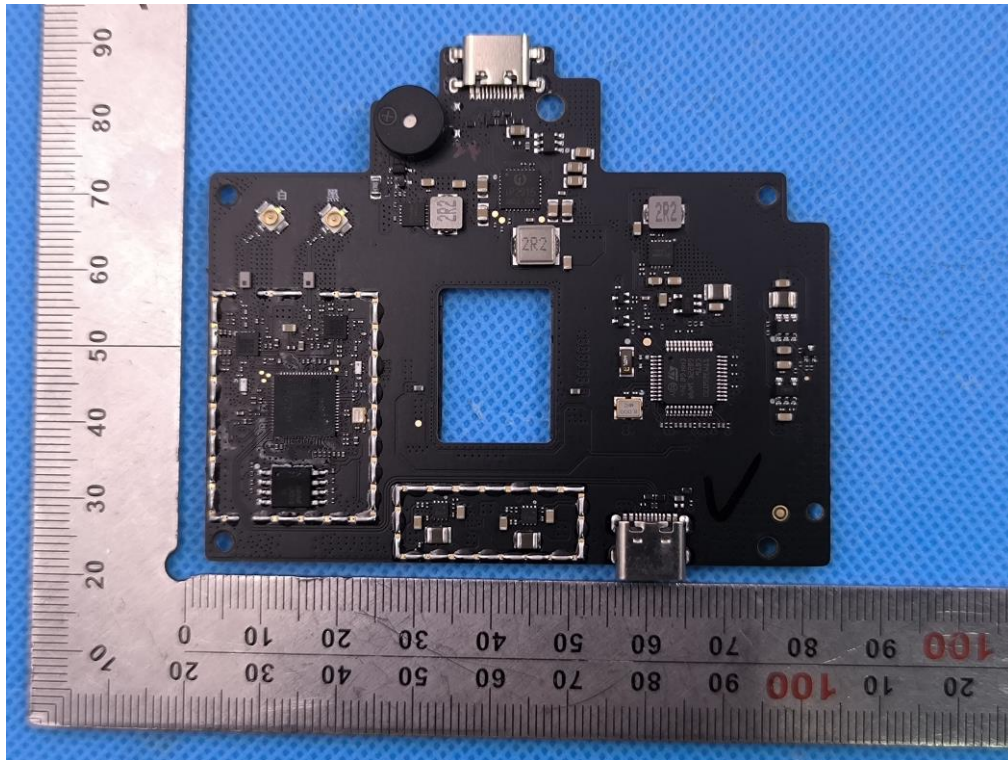
INTERNAL VIEW OF EUT-1 (FIGURE 3)
