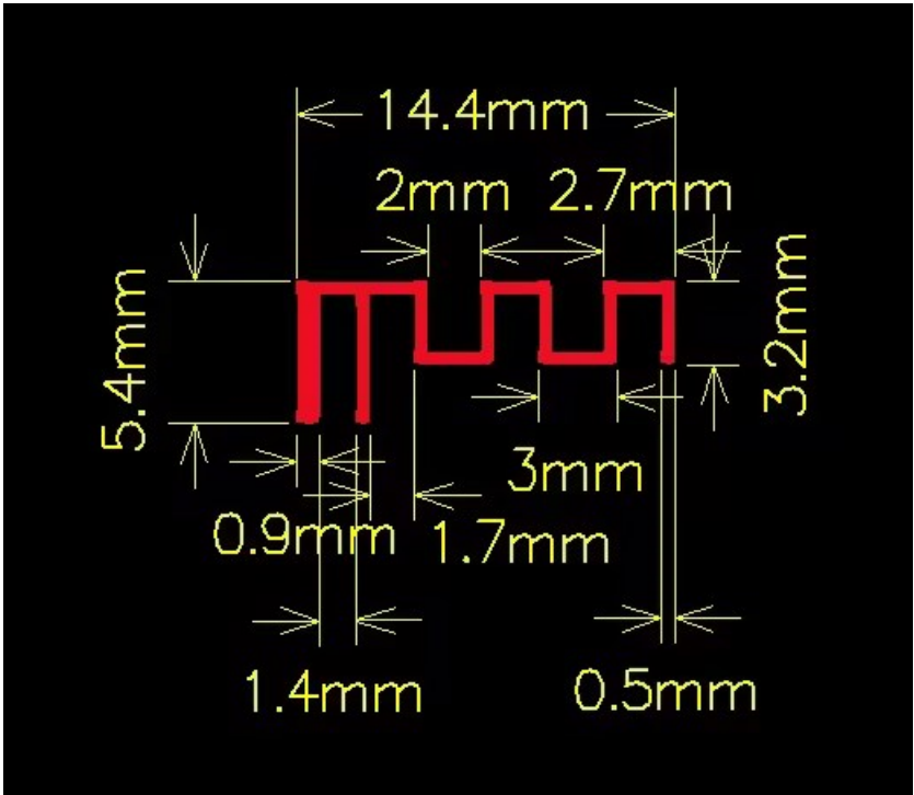
Picture of antenna
