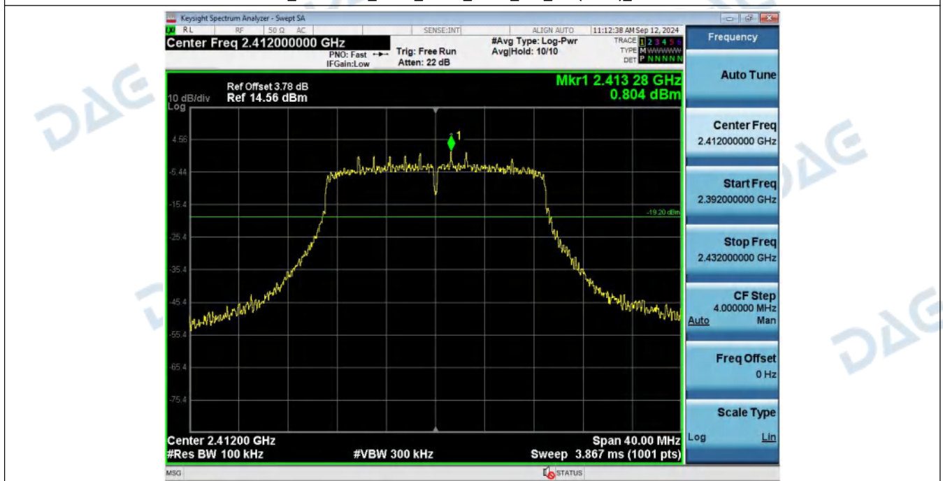
2_Bandedge_NVNT_ANT1_802_11n(HT20)_2412
