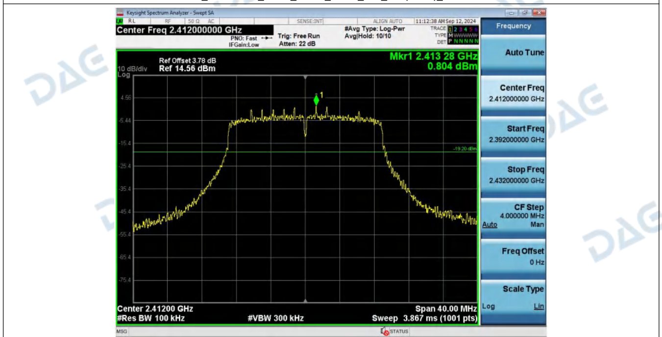
2_Spurious_Emission_NVNT_ANT1_802_11n(HT20)_2412
