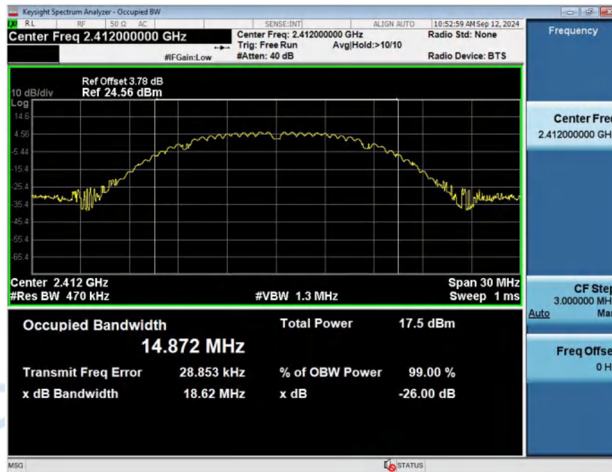
99%_Occupied_Bandwidth_NVNT_ANT1_802_11b_2412
