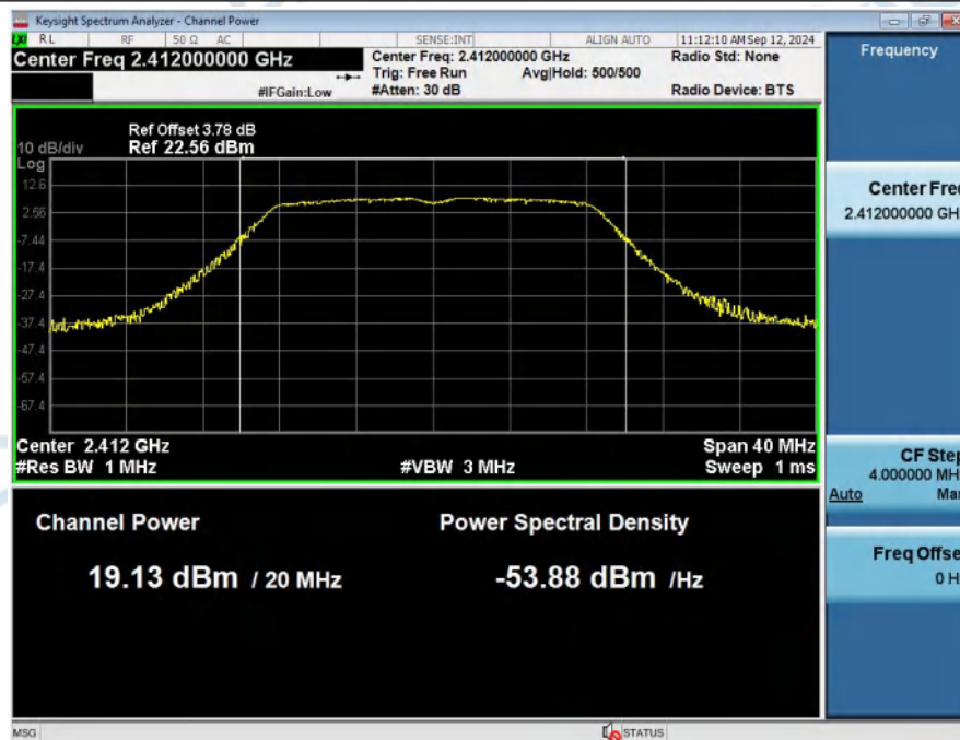
MAX__Output_Power_NVNT_ANT1_802_11n(HT20)_2412
