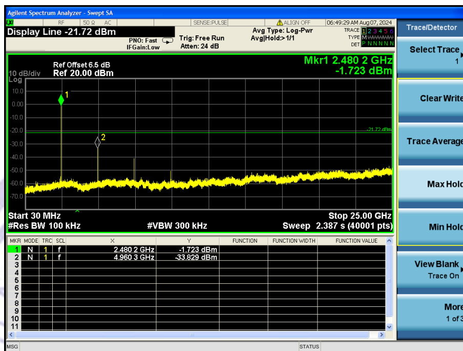
BLE-2M
