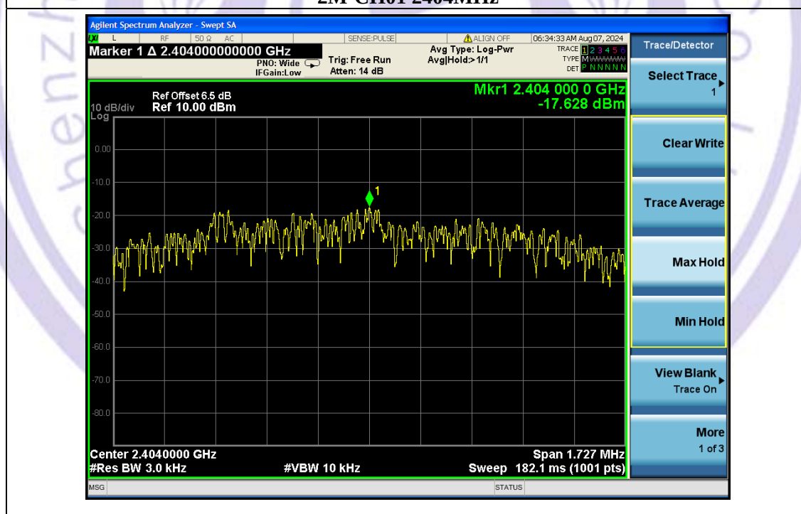
2M-CH01 2404MHz
