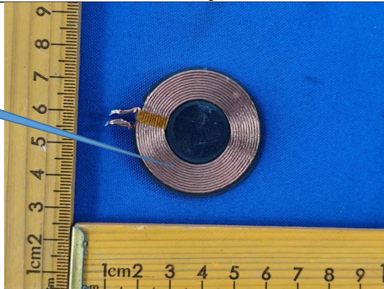
Coil ANT
