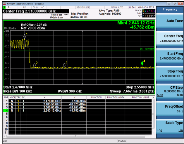
DH5-Ant1-Hop_2480-PASS
