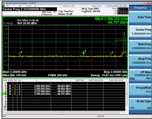
2DH5-Ant1-2402-PASS
