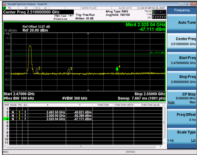
2DH5-Ant1-2480-PASS
