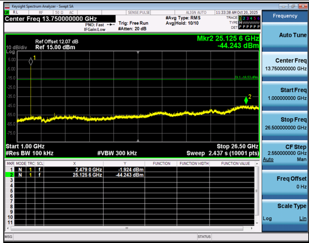
3DH5-Ant1-2480-1000~26500-PASS
