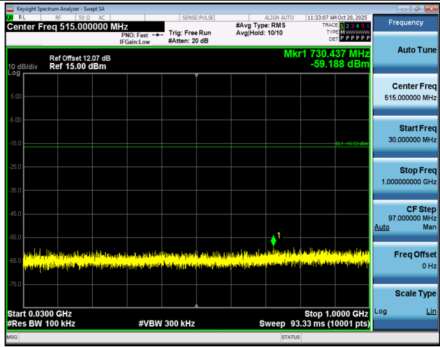
3DH5-Ant1-2480-30~1000-PASS
