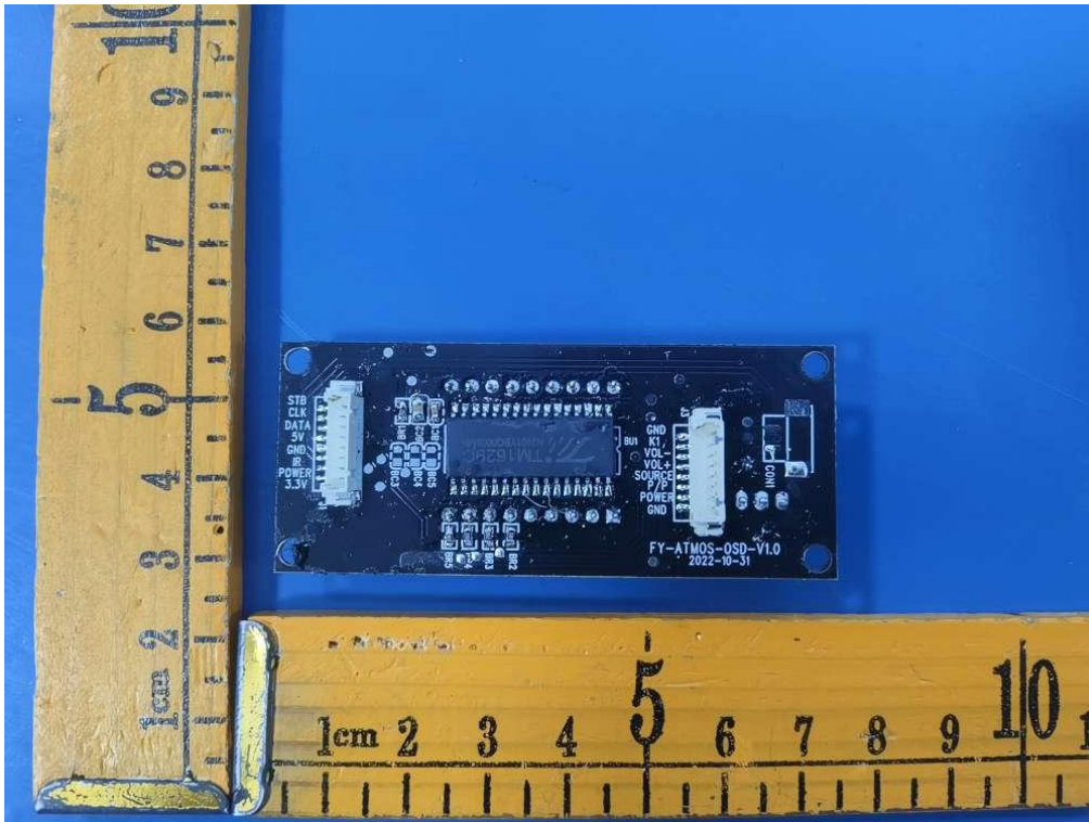
Internal view of unit (Model:D51W, D71W)
