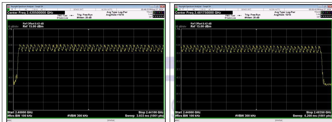
Low End Spectrum Channel Hopping Plot 8DPSK
