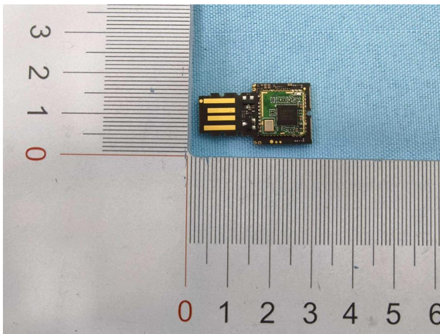
WiFi ANT
