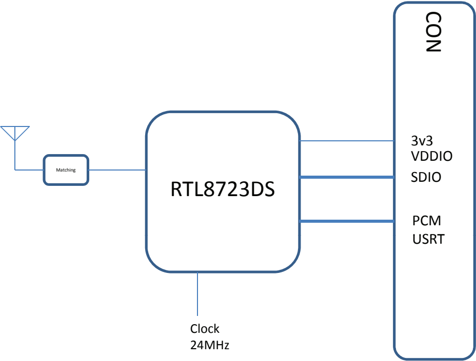
6223A-SRD Block Diagram
