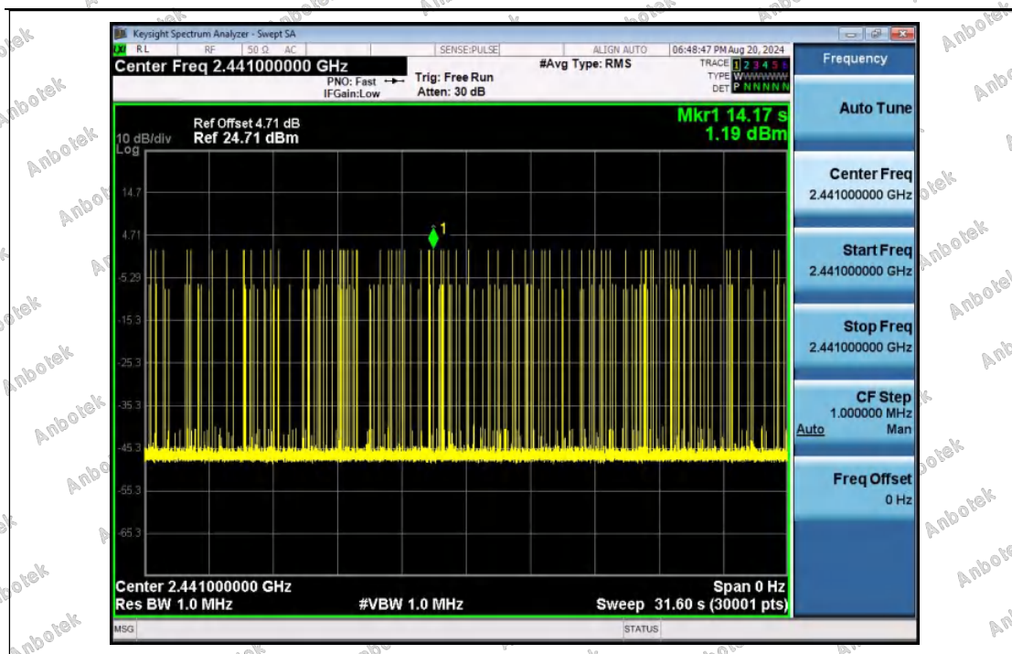
Dwell_Time_(Hopping)_NVNT_ANT1_2-DH1_2441_00_One_Burst_Time
