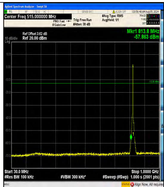
Band5_5MHz_16QAM_20425_25RB#0_30~100 0 30~1000
