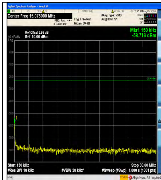
Band5_5MHz_16QAM_20425_25RB#0_0.15~30 0.15~30
