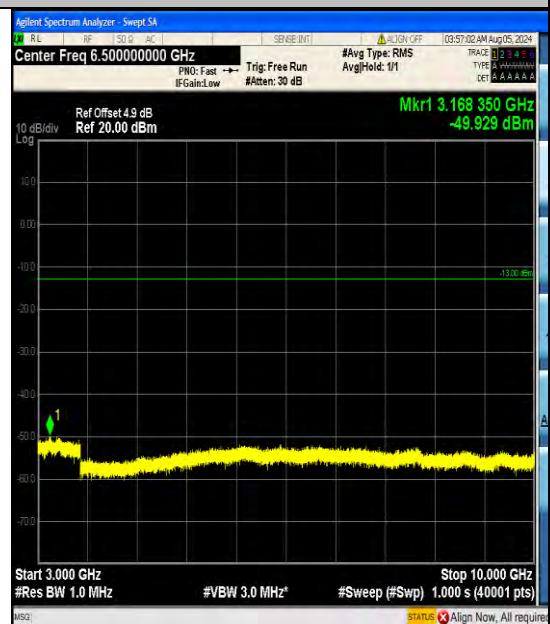
Band5_5MHz_16QAM_20425_25RB#0_3000~10000_3000~10000
