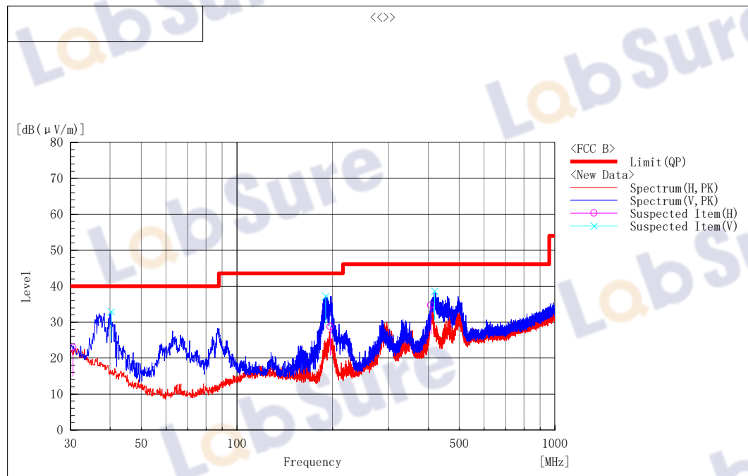
Spectrum Selection
