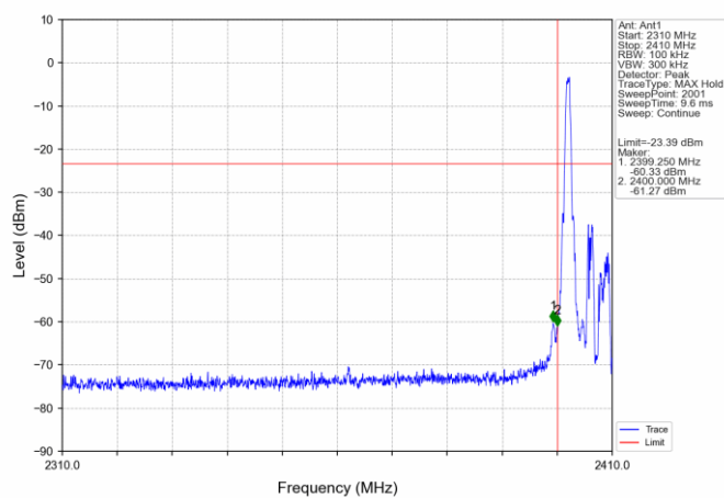
1M_LCH_2402MHz_Ant1_NTNV
