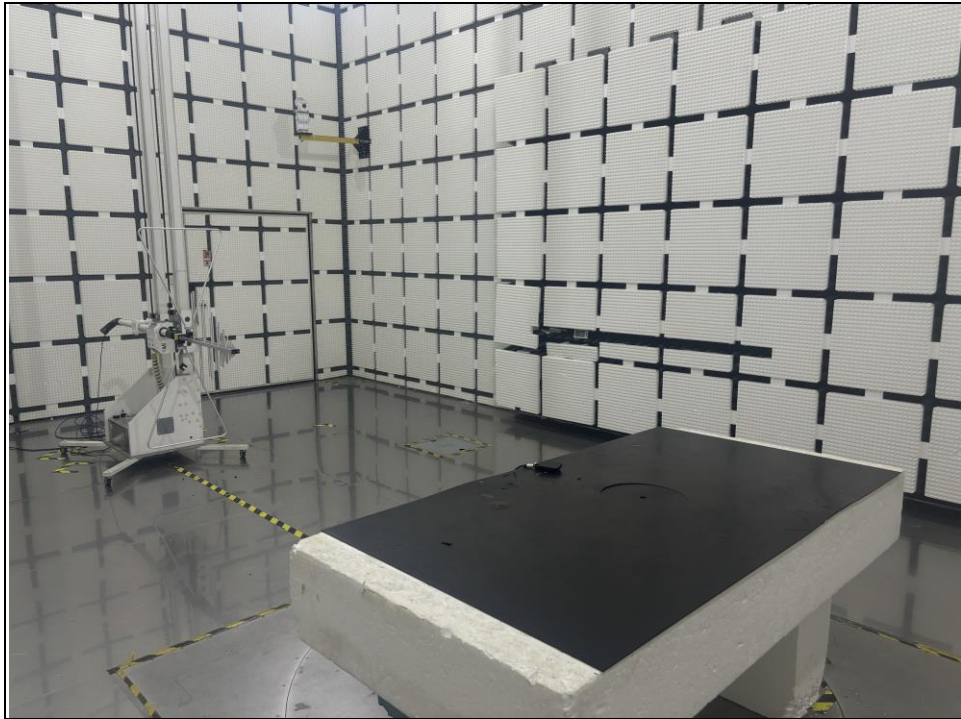
SPURIOUS EMISSION TEST-1
