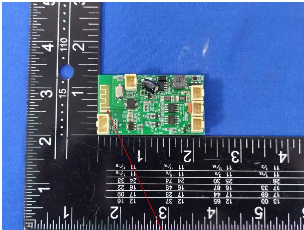
PCB ANTENNA
