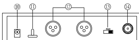
Painel frontal
