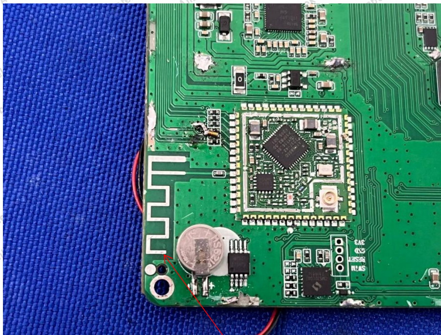
WIFI 2.4G ANT(no use, function has been blocked by software)
