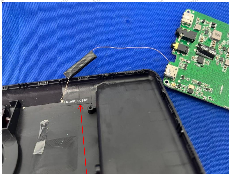
FM ANT(no use, function has been blocked by software)
