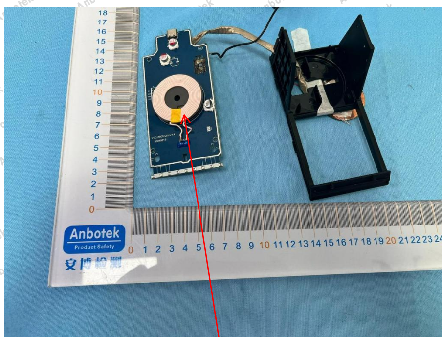
Earphone-ANT
