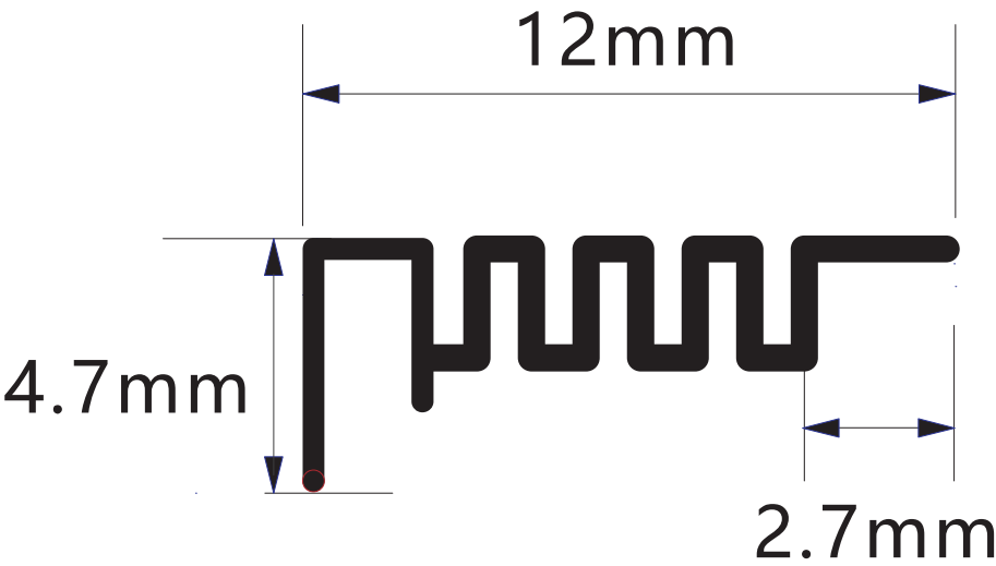
Antenna Photo & Length (mm)
