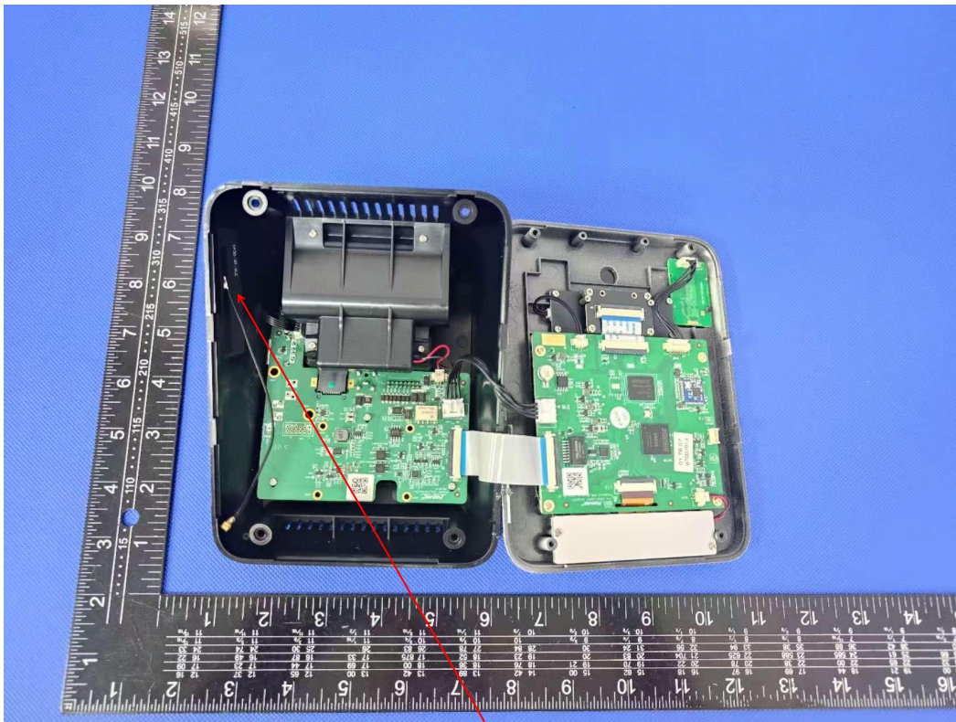
WIFI ANT
