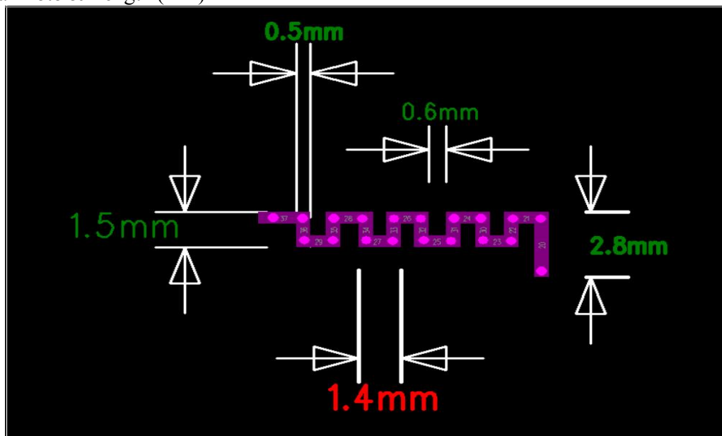
Antenna Photo & Length (mm)
