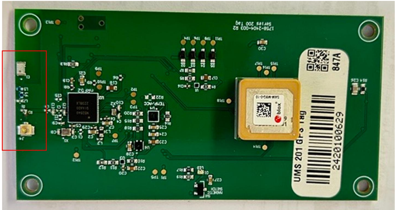
ISM Transmitter Path and uFL port for Patch Antenna Location
