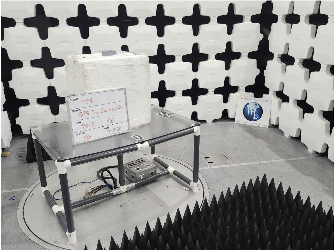
RE >1GHz, View 2
