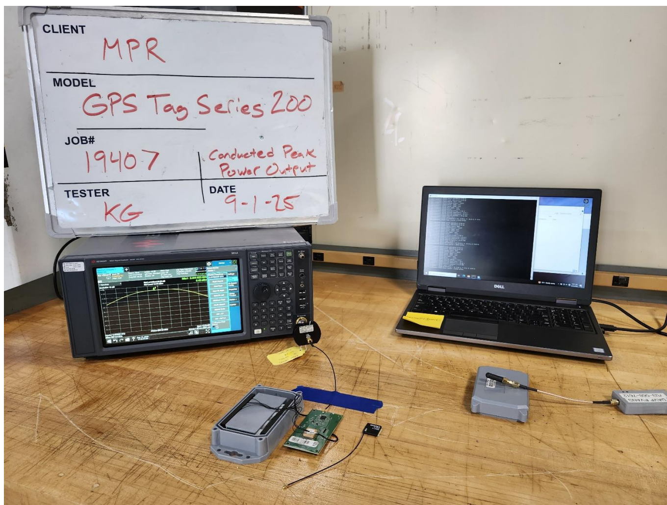
Conducted Antenna Port
