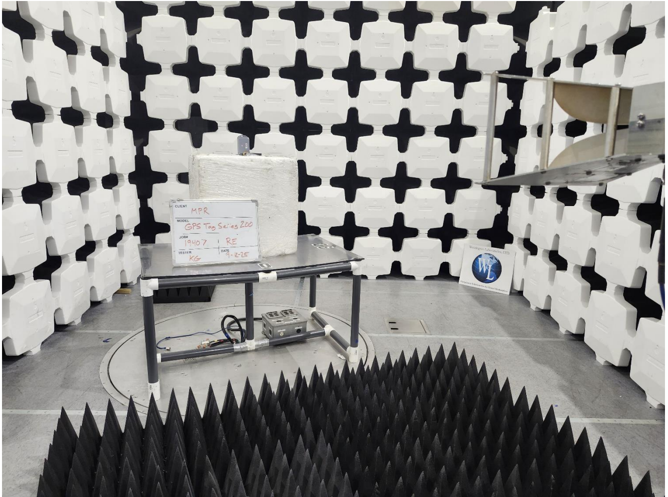
RE >1GHz, View 1
