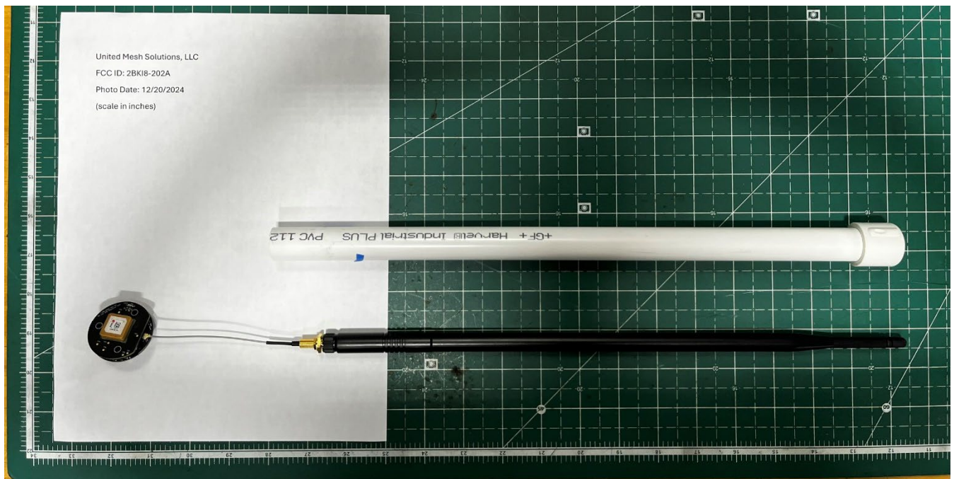
TX Antenna Assembly
