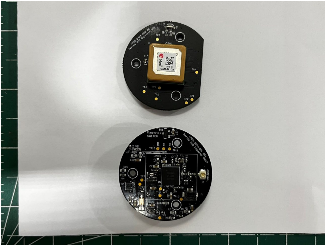
PCB Deconstructed View
