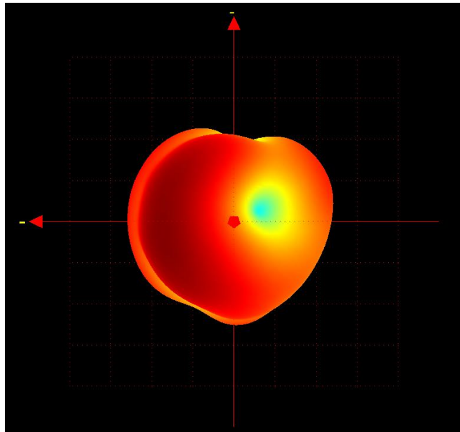
(4) Typical Free Space 3D Radiation Pattern at 2.44GMHz:
