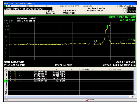
Out Of Band Emission IEEE 802.11ac_Channel 48_20MHz_Antenna 0
