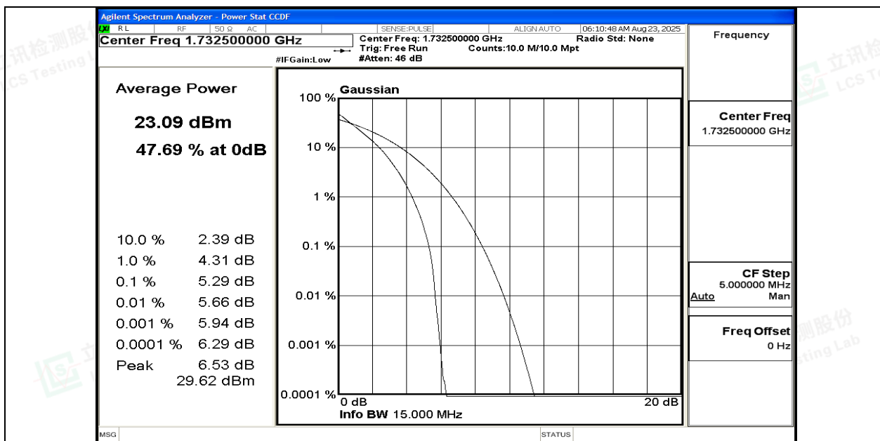
Band4-15MHz-QPSK-20175-75RB#0-PASS
