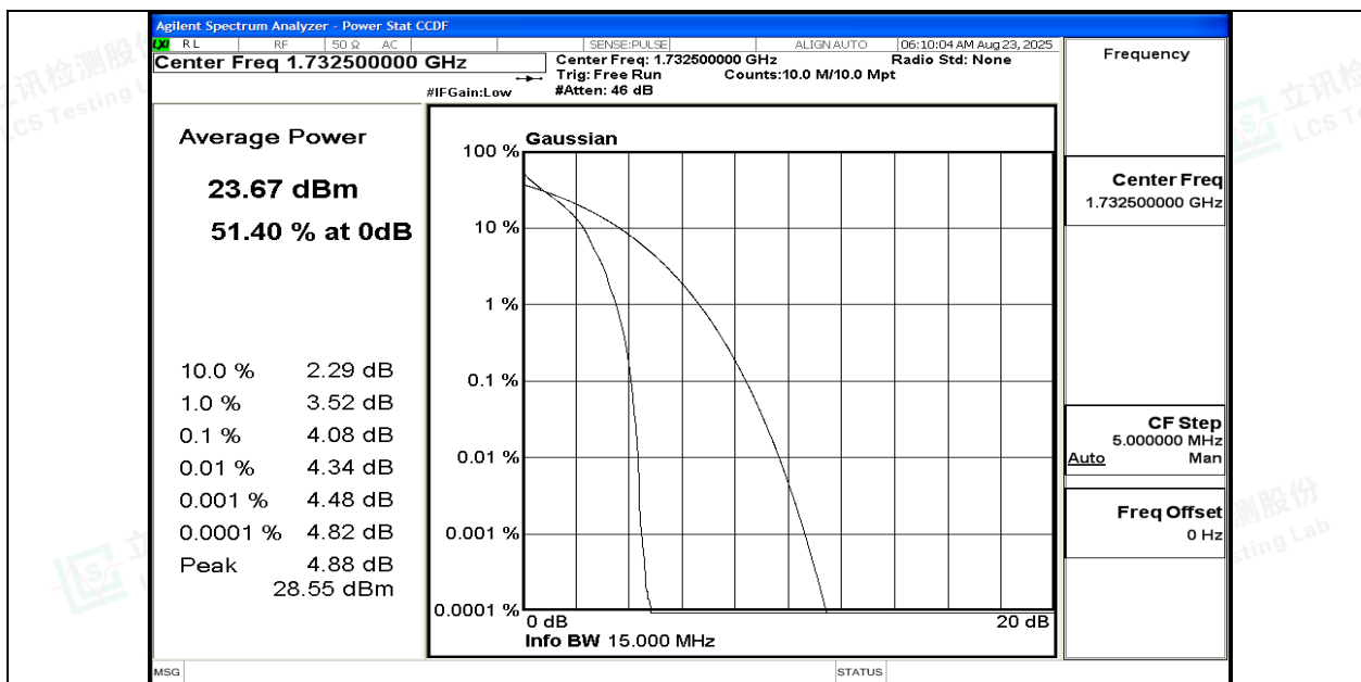
Band4-15MHz-QPSK-20175-1RB#0-PASS
