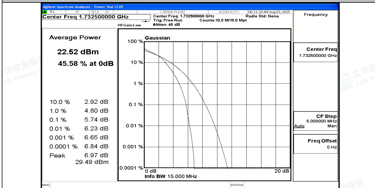
Band4-15MHz-16QAM-20175-75RB#0-PASS
