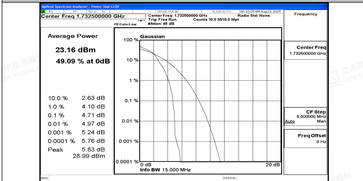
Band4-15MHz-16QAM-20175-1RB#0-PASS
