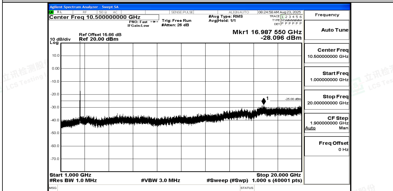
Band7_10MHz_QPSK_21100_1RB#0_1000~20000_1000~20000
