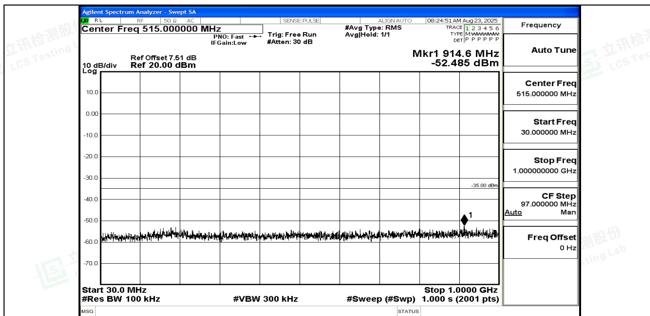
Band7_10MHz_QPSK_21100_1RB#0_30~1000_30~1000
