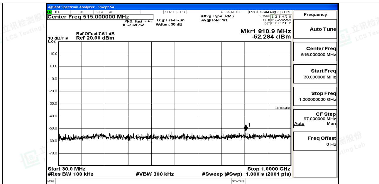
Band7_20MHz_QPSK_21350_1RB#0_30~1000_30~1000
