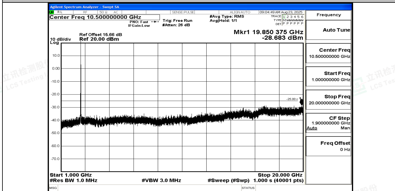
Band7_20MHz_QPSK_21350_1RB#0_1000~20000_1000~20000
