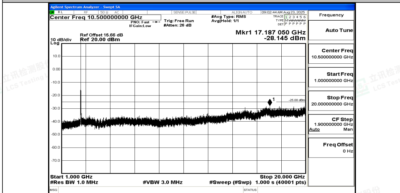
Band7_20MHz_QPSK_20850_1RB#0_1000~20000_1000~20000
