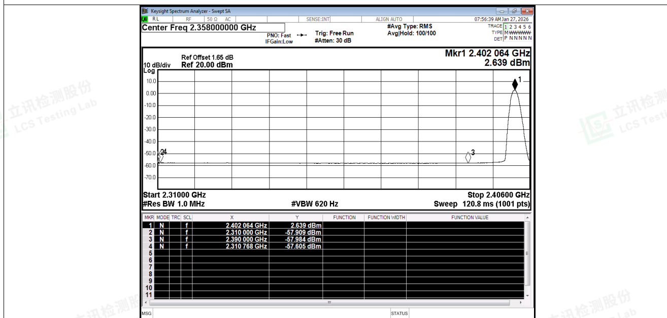
Restrict Band NVNT BLE 1M 2402MHz Ant1 Average
