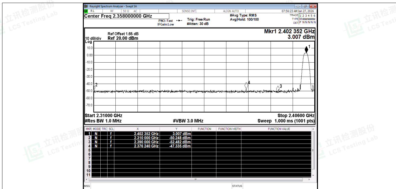
Restrict Band NVNT BLE 1M 2402MHz Ant1 Peak
