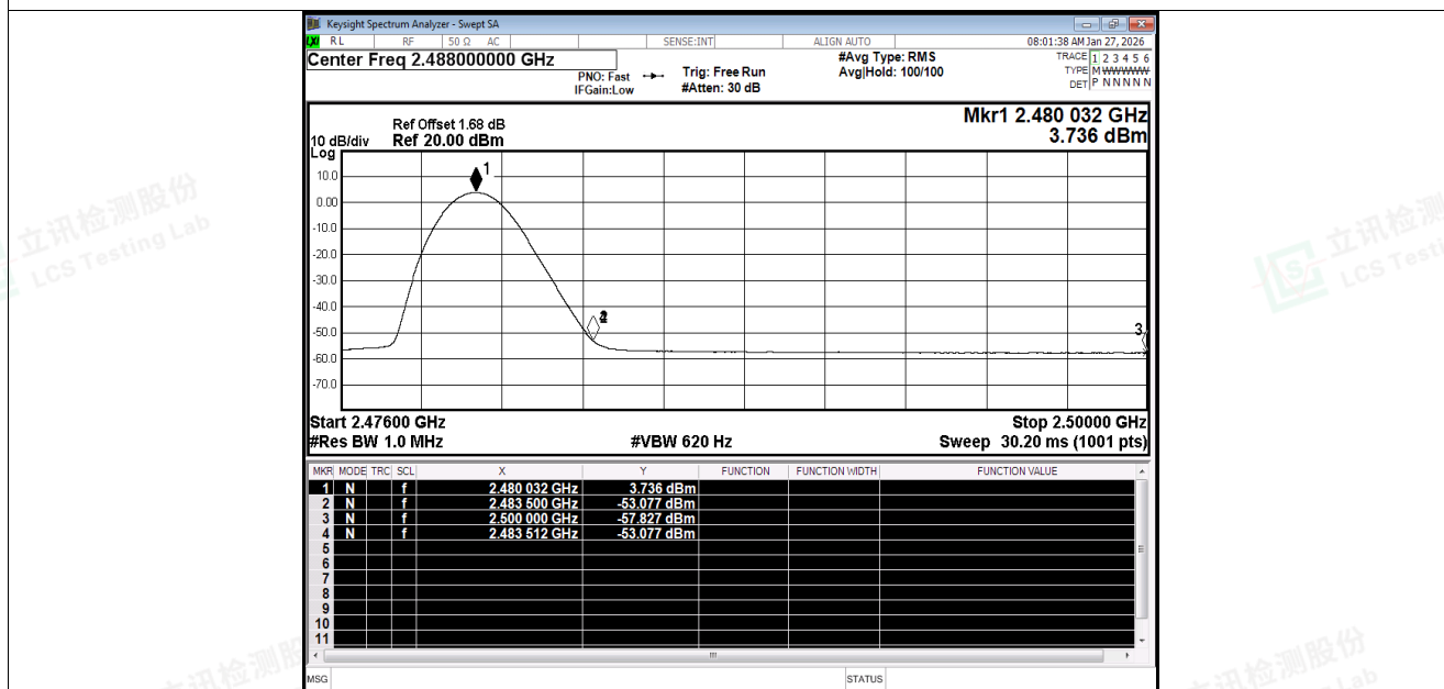
Restrict Band NVNT BLE 1M 2480MHz Ant1 Average
