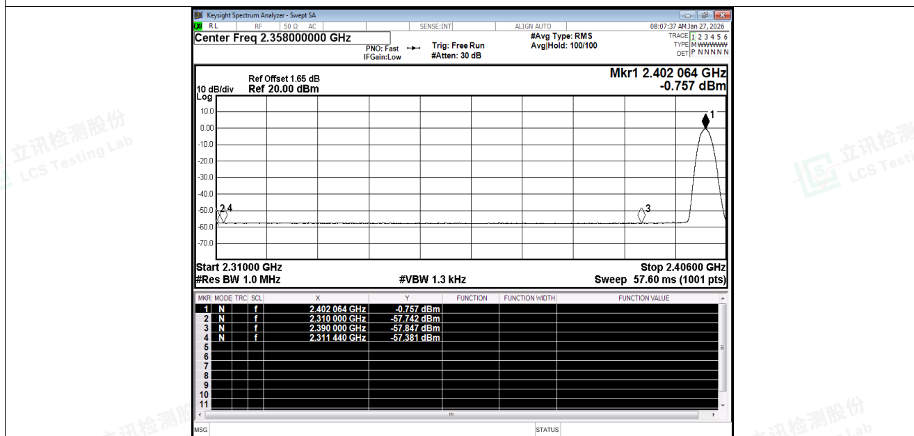
Restrict Band NVNT BLE 2M 2402MHz Ant1 Average
