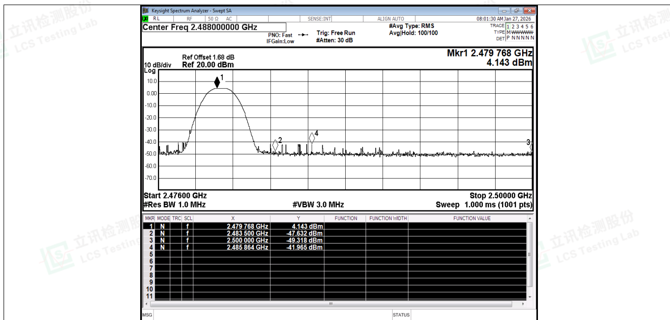
Restrict Band NVNT BLE 1M 2480MHz Ant1 Peak
