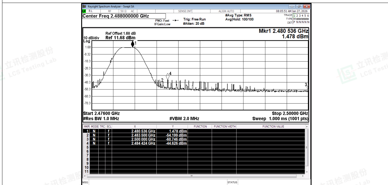
Restrict Band NVNT BLE 2M 2480MHz Ant1 Average
