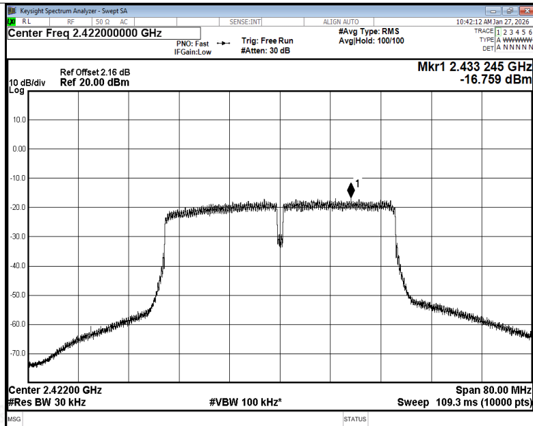
PSD NVNT n40 2422MHz Ant1
