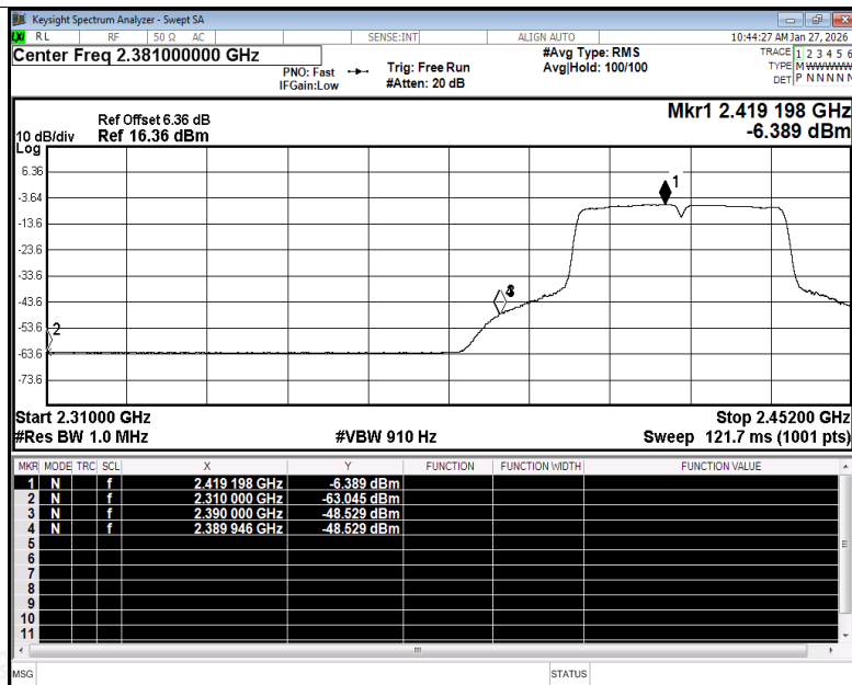
Restrict Band NVNT n40 2422MHz Ant1 Average
