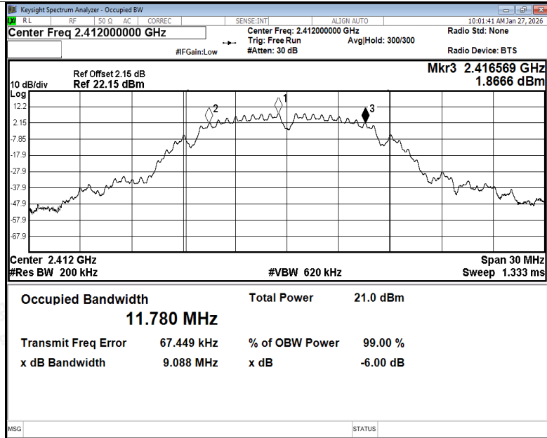
-6dB Bandwidth NVNT b 2412MHz Ant1
