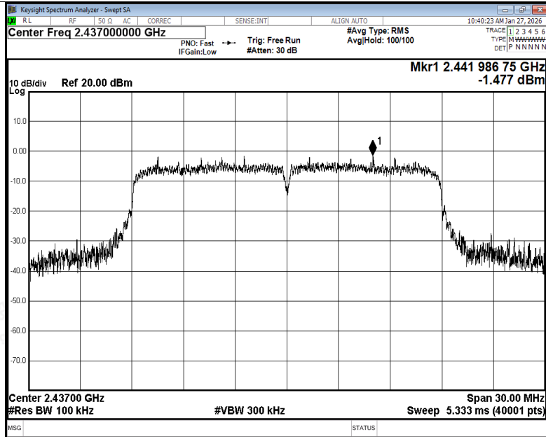
Tx. Spurious NVNT n20 2437MHz Ant1 Ref
