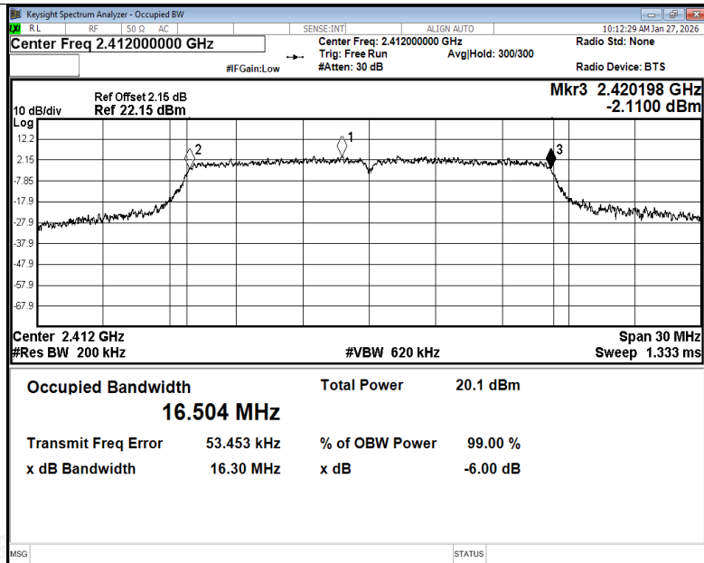
-6dB Bandwidth NVNT g 2412MHz Ant1
