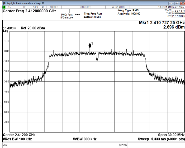
Tx. Spurious NVNT g 2412MHz Ant1 Ref
