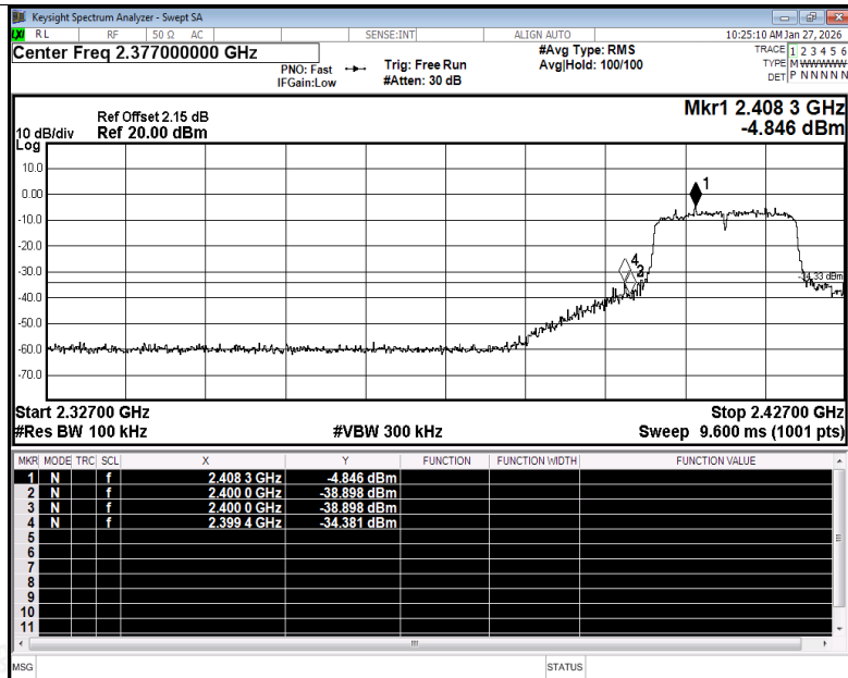
Band Edge NVNT n20 2412MHz Ant1 Emission
