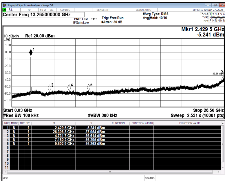
Tx. Spurious NVNT n40 2422MHz Ant1 Emission
