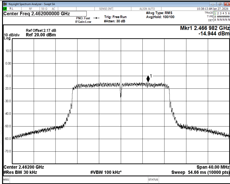
PSD NVNT n20 2462MHz Ant1
