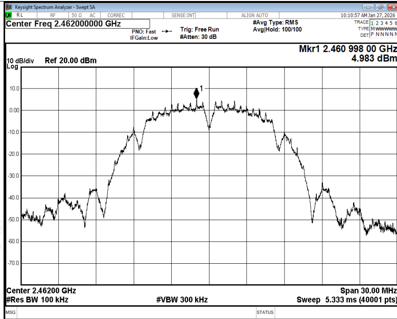
Tx. Spurious NVNT b 2462MHz Ant1 Ref
