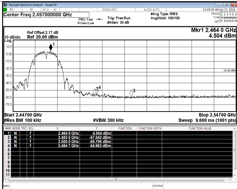
Band Edge NVNT b 2462MHz Ant1 Emission
