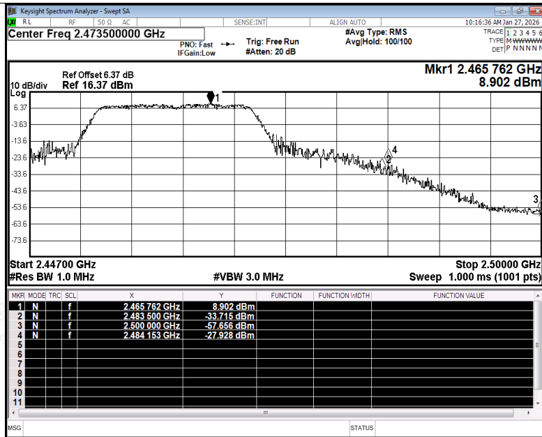
Restrict Band NVNT g 2462MHz Ant1 Peak
