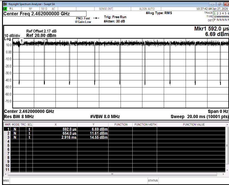
Duty Cycle NVNT n20 2462MHz Ant1
