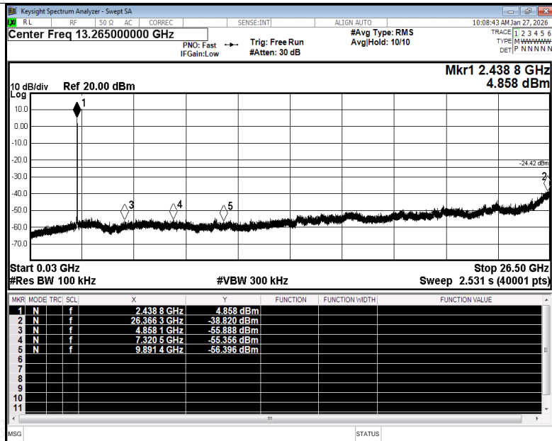
Tx. Spurious NVNT b 2437MHz Ant1 Emission
