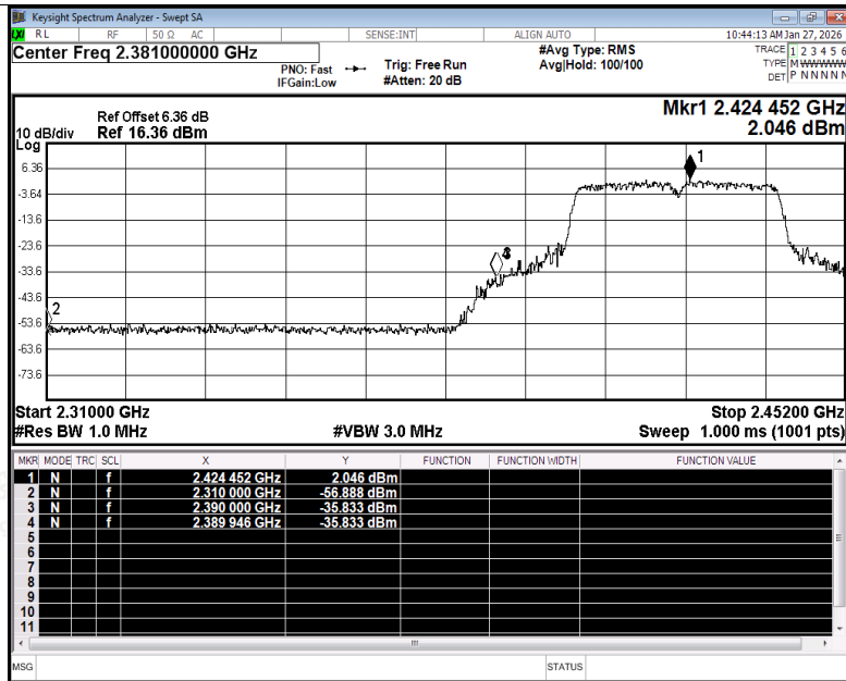
Restrict Band NVNT n40 2422MHz Ant1 Peak
