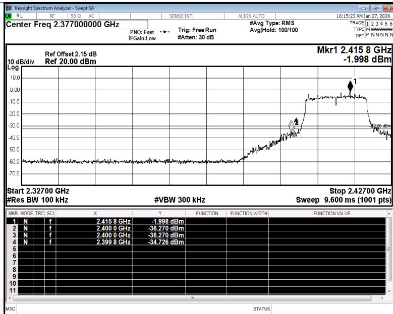
Band Edge NVNT g 2412MHz Ant1 Emission
