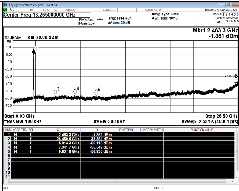
Tx. Spurious NVNT n20 2462MHz Ant1 Emission
