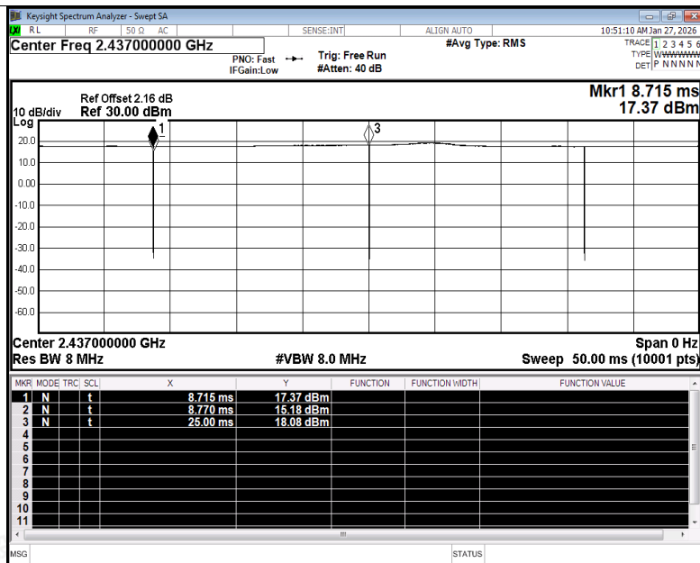
Duty Cycle NVNT b 2437MHz Ant1
