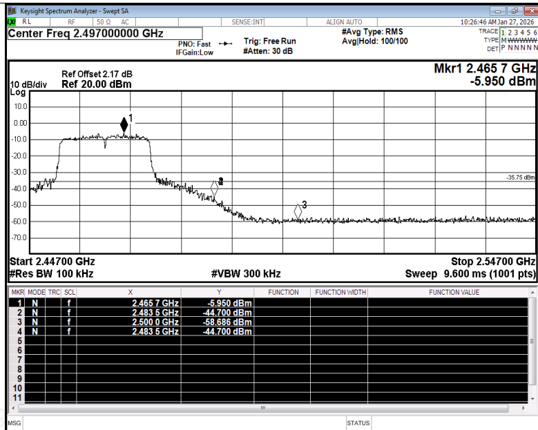
Band Edge NVNT n20 2462MHz Ant1 Emission
