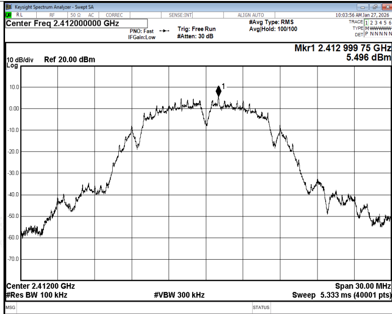
Tx. Spurious NVNT b 2412MHz Ant1 Ref
