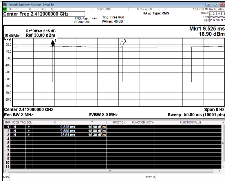
Duty Cycle NVNT b 2412MHz Ant1
