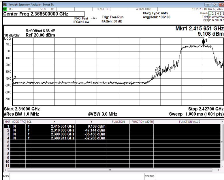
Restrict Band NVNT n20 2412MHz Ant1 Peak
