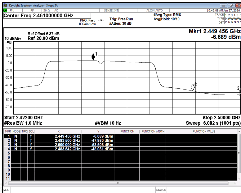
Restrict Band NVNT n40 2452MHz Ant1 Average
