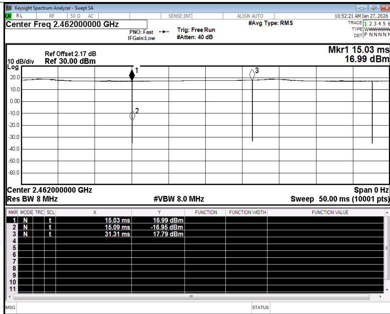
Duty Cycle NVNT b 2462MHz Ant1
