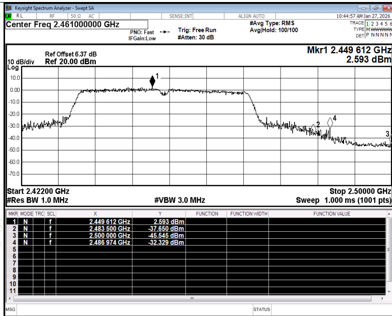
Restrict Band NVNT n40 2452MHz Ant1 Peak
