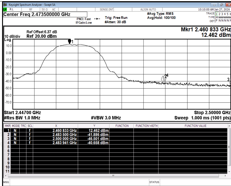
Restrict Band NVNT b 2462MHz Ant1 Peak
