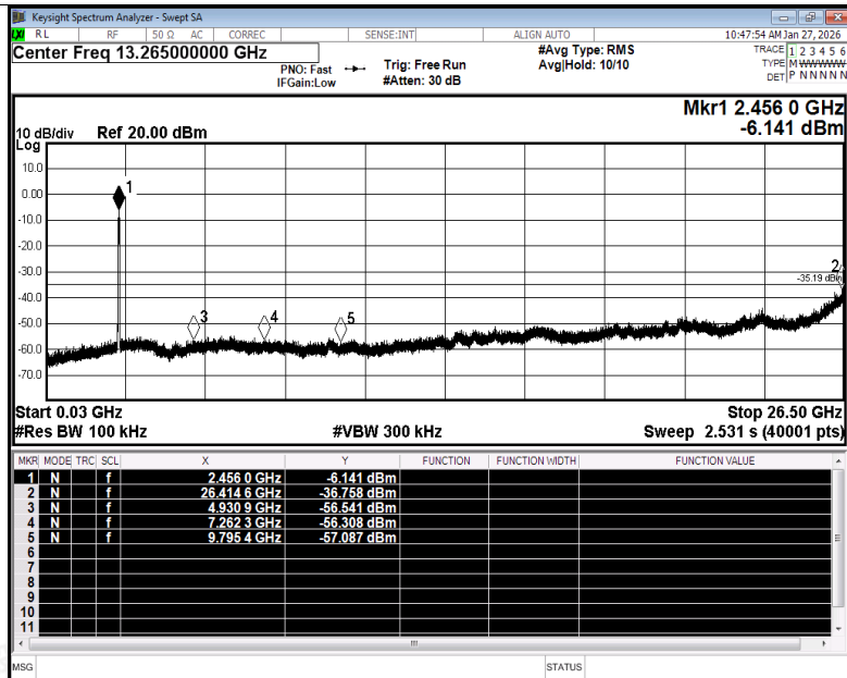
Tx. Spurious NVNT n40 2452MHz Ant1 Emission
