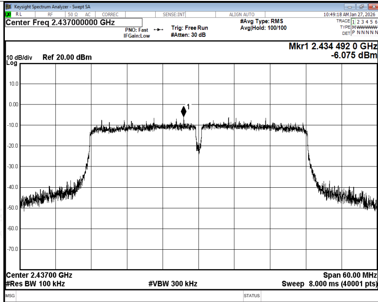
Tx. Spurious NVNT n40 2437MHz Ant1 Ref
