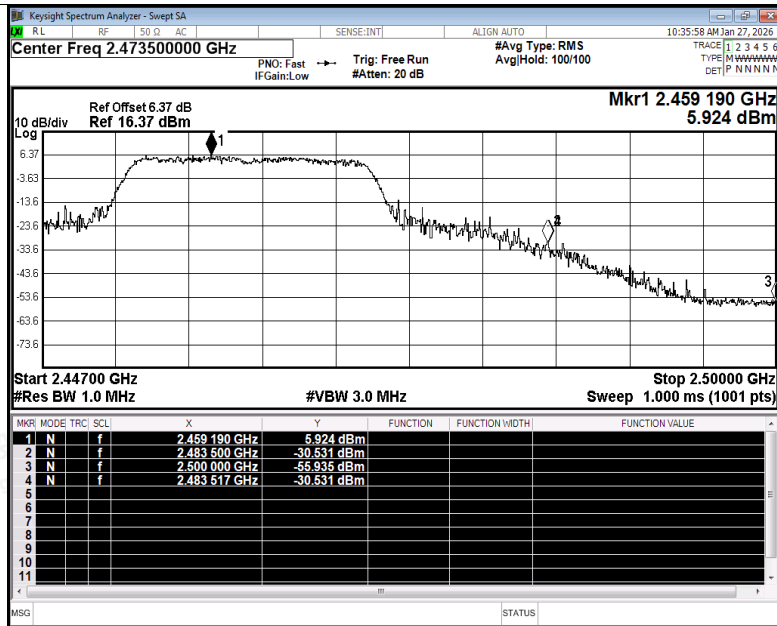
Restrict Band NVNT n20 2462MHz Ant1 Peak
