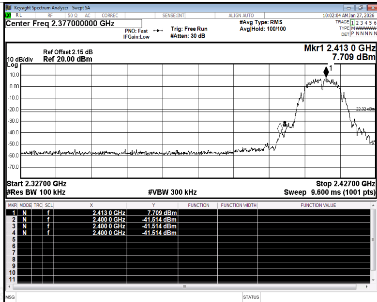
Band Edge NVNT b 2412MHz Ant1 Emission
