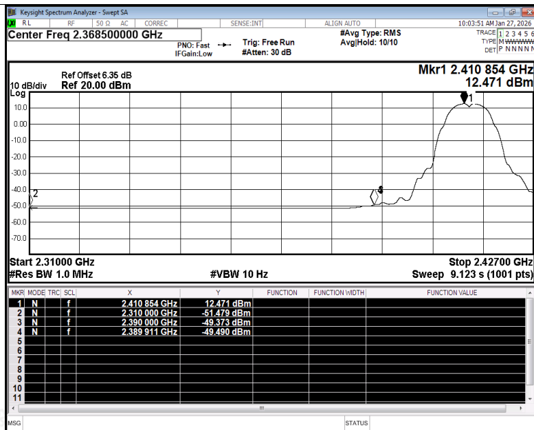
Restrict Band NVNT b 2412MHz Ant1 Average
