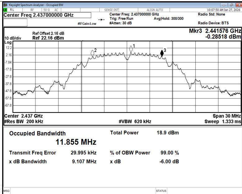
-6dB Bandwidth NVNT b 2437MHz Ant1
