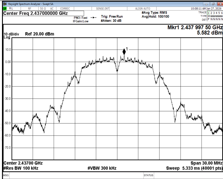
Tx. Spurious NVNT b 2437MHz Ant1 Ref
