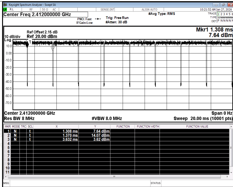
Duty Cycle NVNT n20 2412MHz Ant1
