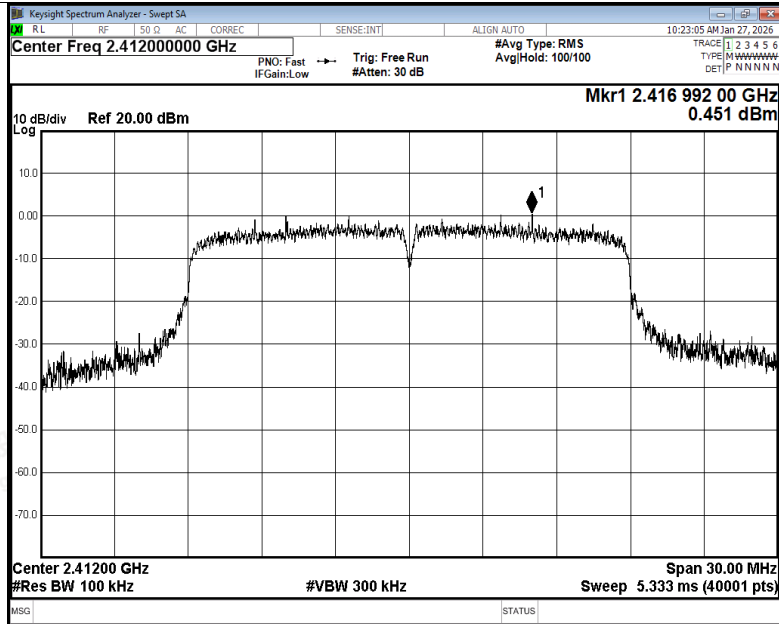
Tx. Spurious NVNT n20 2412MHz Ant1 Ref
