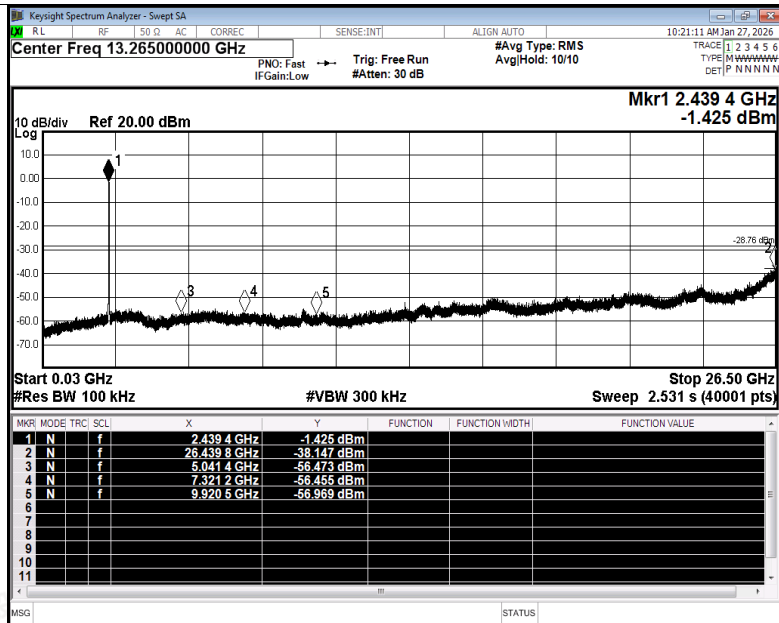
Tx. Spurious NVNT g 2437MHz Ant1 Emission
