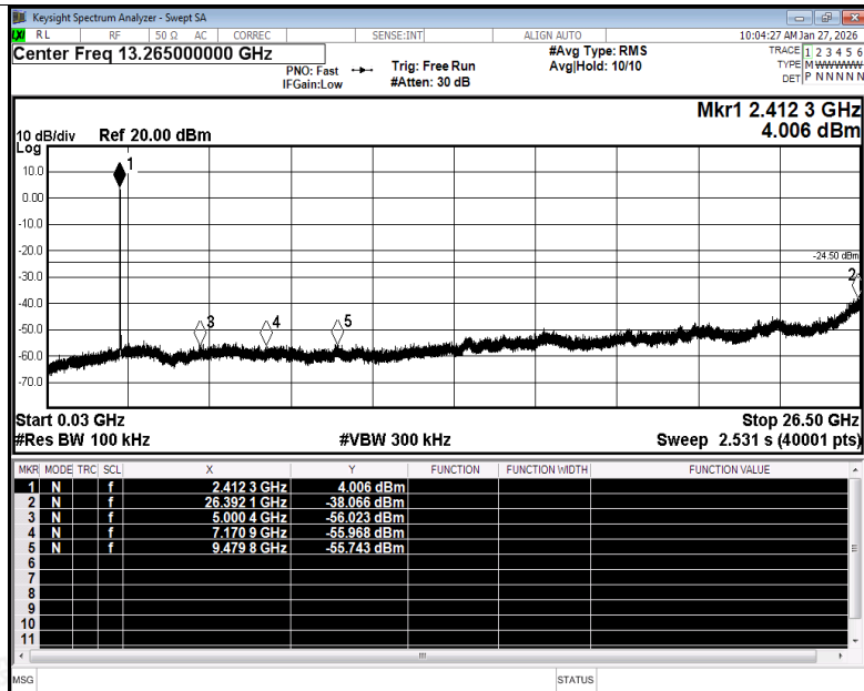
Tx. Spurious NVNT b 2412MHz Ant1 Emission
