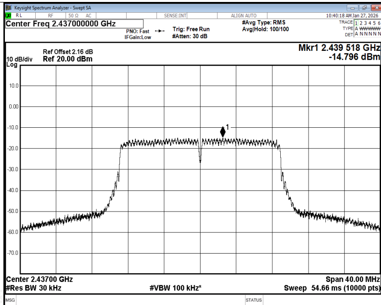
PSD NVNT n20 2437MHz Ant1
