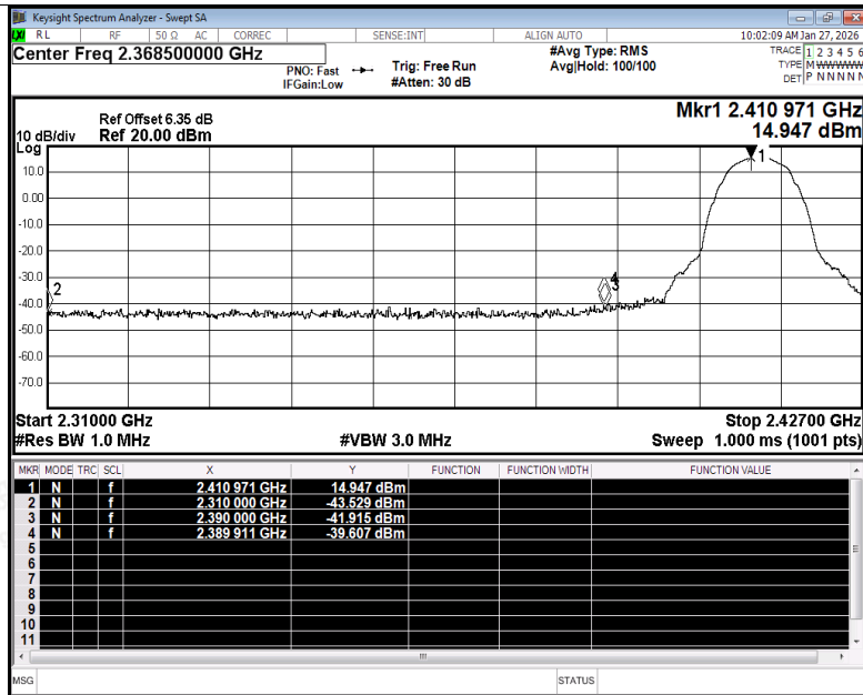
Restrict Band NVNT b 2412MHz Ant1 Peak
