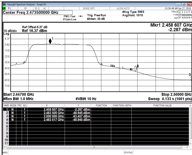
Restrict Band NVNT n20 2462MHz Ant1 Average
