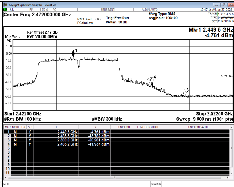
Band Edge NVNT n40 2452MHz Ant1 Emission
