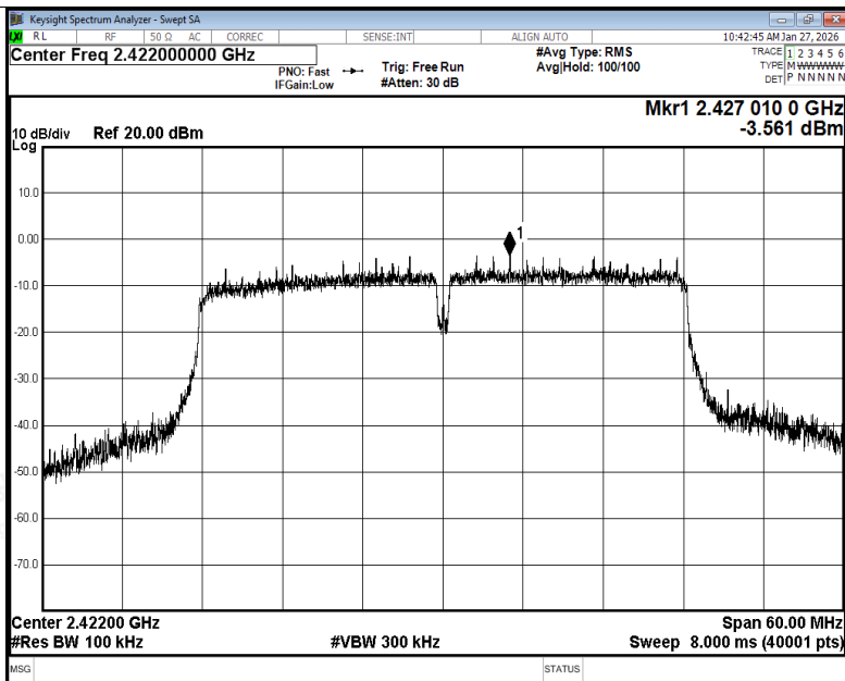
Tx. Spurious NVNT n40 2422MHz Ant1 Ref
