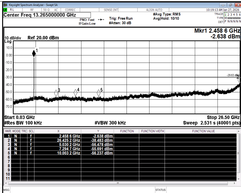
Tx. Spurious NVNT g 2462MHz Ant1 Emission
