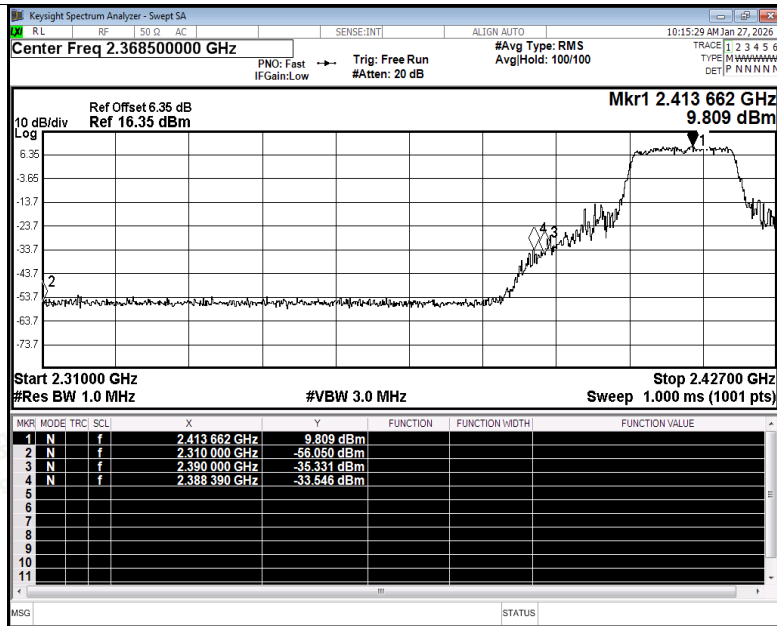
Restrict Band NVNT g 2412MHz Ant1 Peak
