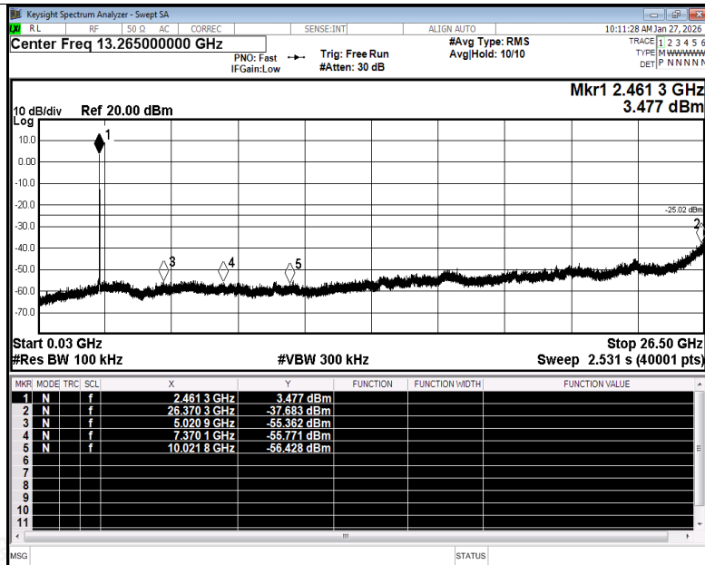
Tx. Spurious NVNT b 2462MHz Ant1 Emission
