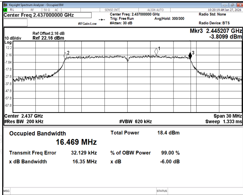
-6dB Bandwidth NVNT g 2437MHz Ant1
