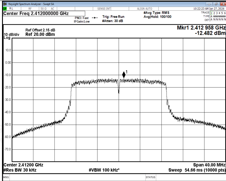
PSD NVNT n20 2412MHz Ant1
