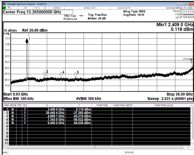
Tx. Spurious NVNT g 2412MHz Ant1 Emission
