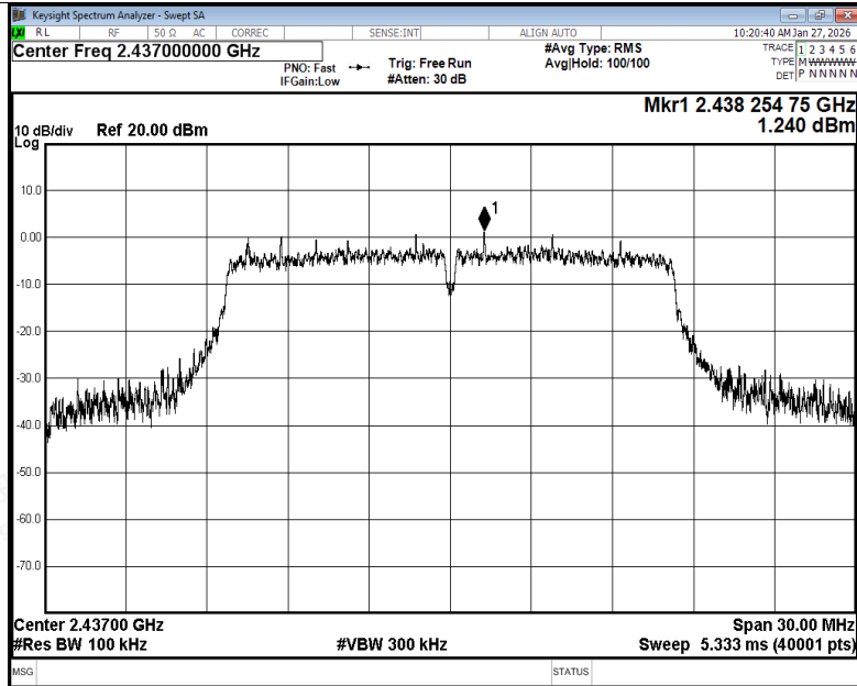
Tx. Spurious NVNT g 2437MHz Ant1 Ref
