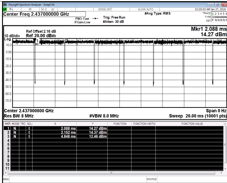
Duty Cycle NVNT g 2437MHz Ant1
