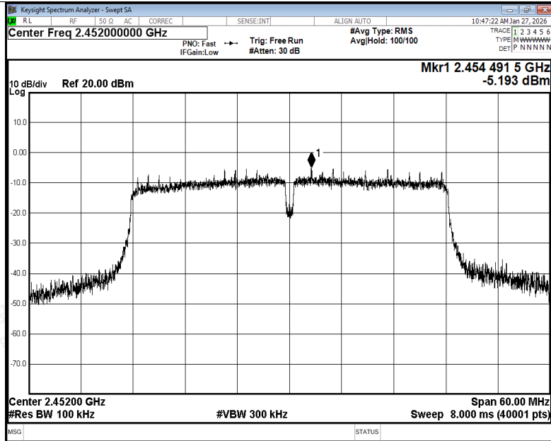
Tx. Spurious NVNT n40 2452MHz Ant1 Ref
