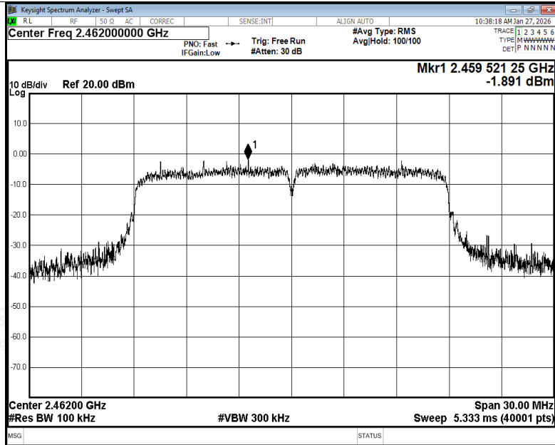
Tx. Spurious NVNT n20 2462MHz Ant1 Ref
