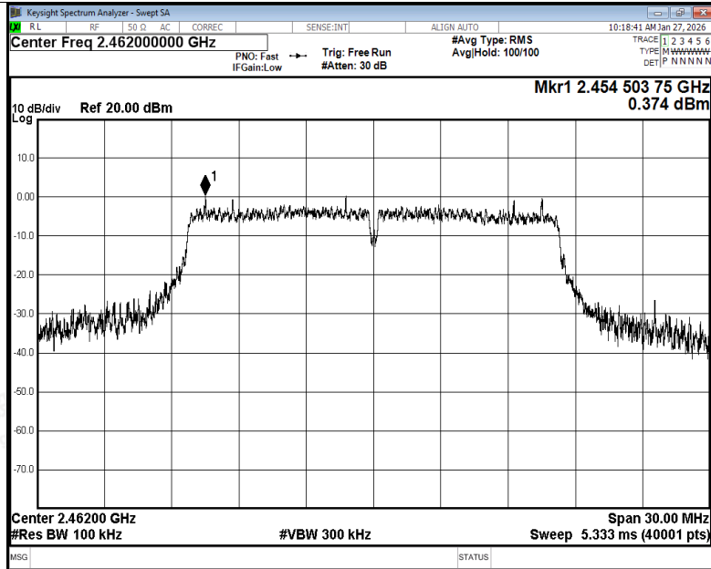
Tx. Spurious NVNT g 2462MHz Ant1 Ref
