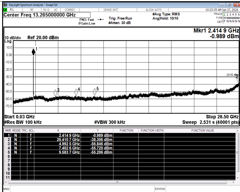
Tx. Spurious NVNT n20 2412MHz Ant1 Emission
