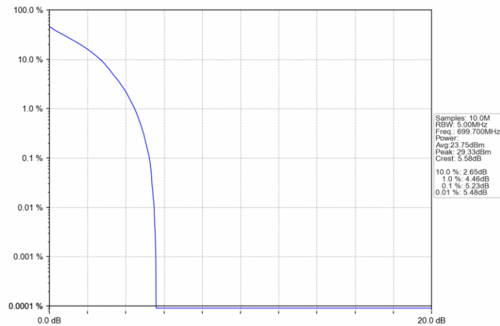
Band12_1.4MHz_QPSK_LCH_699.7MHz_RB_6_0_NTNV
