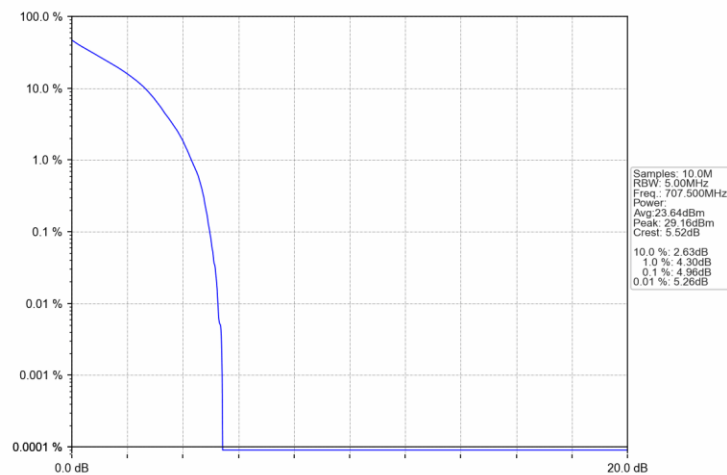
Band12_1.4MHz_QPSK_MCH_707.5MHz_RB_6_0_NTNV
