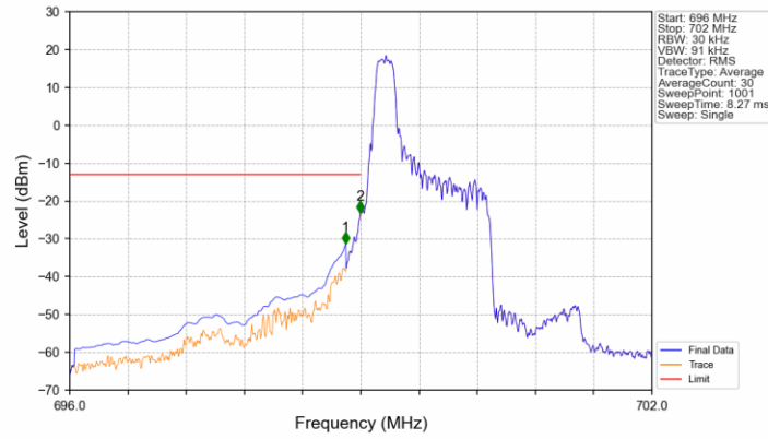
Band12_1.4MHz_QPSK_LCH_699.7MHz_RB_1_0_NTNV
